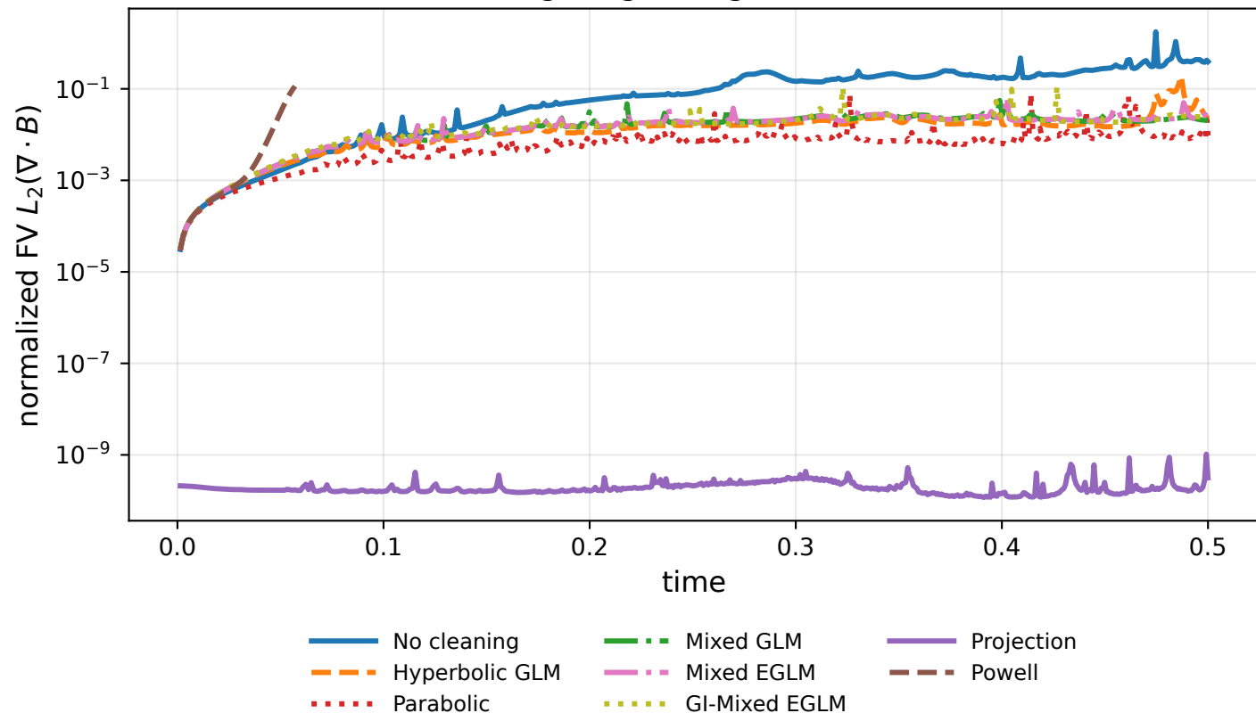
Orszag-Tang divergence control
