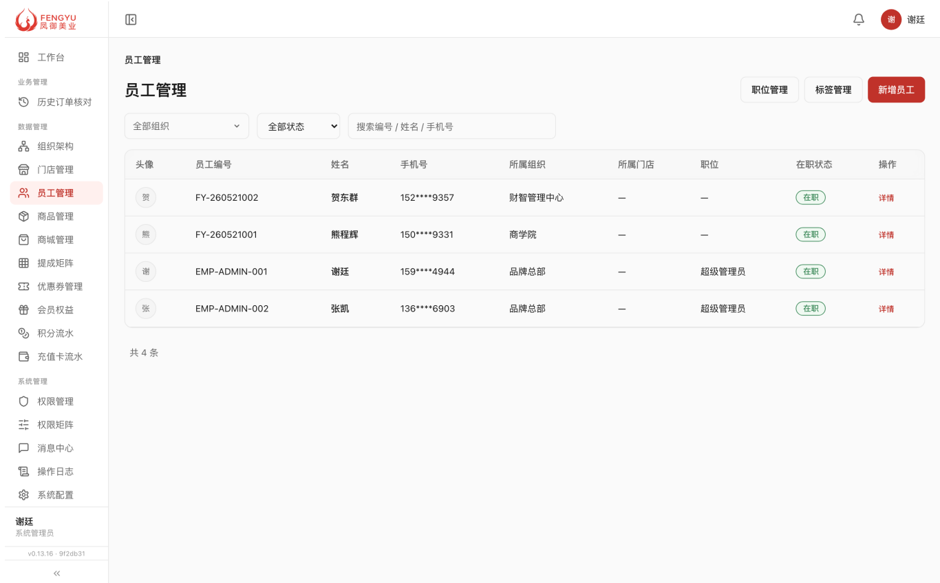
Figure 8: 员工列表页
