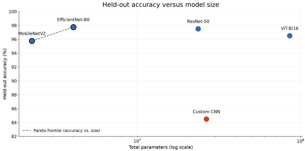
Figure 12: Held-out accuracy against total parameter count (log scale). Circled markers lie on the Pareto frontier: no other model in the study achieves both higher accuracy and a smaller parameter count. ResNet-50, ViT-B/16 and the custom CNN are each dominated by at least one other approach.
