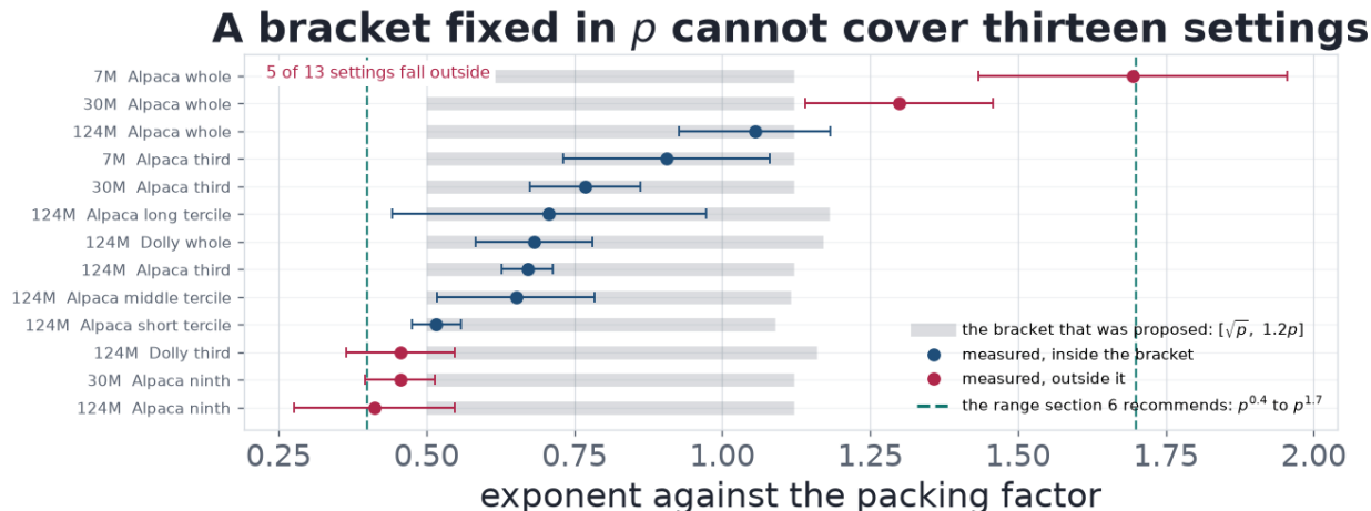
Figure 5: Every one of the thirteen settings against the bracket an earlier draft proposed. In exponent terms that bracket is 0.5 at the floor and \log(1.2p)/\log(p) at the ceiling (about 1.12 to 1.17 over the packing factors here), drawn as the grey band. Five settings fall outside it, and not at random: the three below the floor are the three smallest-scale settings, and the two above the ceiling are the two smaller models on the largest corpus. The dashed verticals are the range this section recommends instead. Error bars are the seed bound of §4.5.
