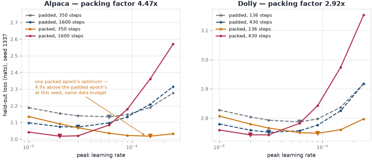
Figure 1: Held-out loss against peak learning rate, seed 1337, minima marked. Dashed is padded, solid is packed. The figure is one seed because the held-out split is seeded with the training seed (3.1); the optima in the tables are aggregated across seeds, each solved on its own curve.
