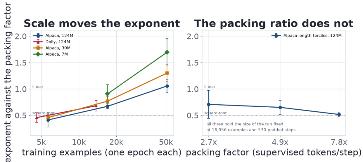
Figure 3: Left: the exponent against the size of the run, with packing factor, padded batch and length distribution held, on both corpora and, from §4.7, at all three model sizes. Every series rises, and the smaller the model the higher it sits, though adjacent models’ bars overlap and only the 124M-to-7M span separates. Right: the exponent against the packing factor across Alpaca’s three length terciles, which hold the size of the run fixed instead. Error bars are the seed bound of §4.5, both cells’ ranges carried through the ratio and so conservative. The right-hand panel is why they are drawn: without them its three points look like a trend.
