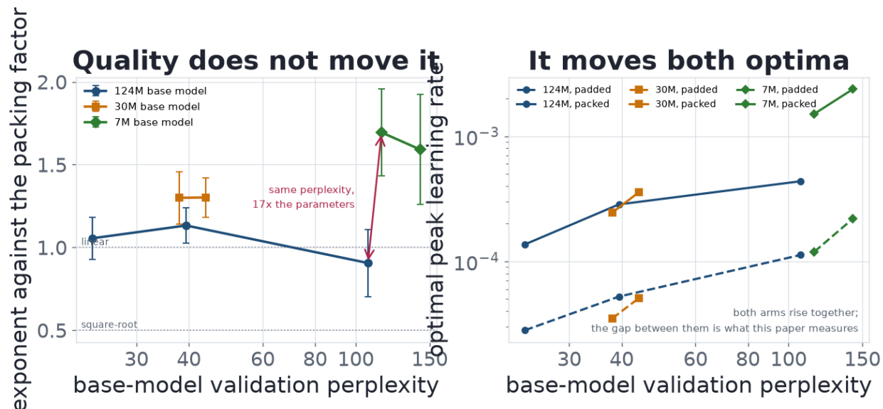
Figure 4: Left: the exponent against the base model’s validation perplexity. The 124M series spans the whole quality range these three models cover and stays flat, while the 7M model sits at the same perplexity as its worst point and more than half an exponent above it. Right: the optima themselves, on the same axis. Both arms rise together as the base model gets worse, by three to four times over this range, while the distance between them is left where it was. Error bars are the seed bound of §4.5; perplexities are read from each model’s own pretraining log.
