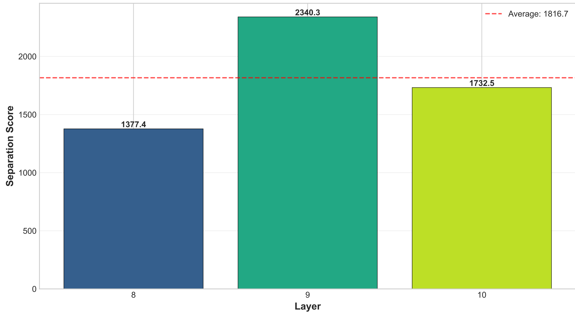
Refusal Direction Separation Across Layers
