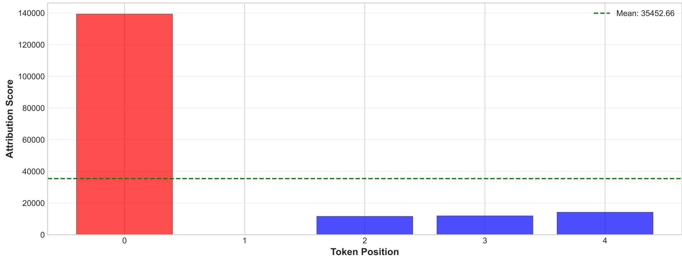
Cumulative Attribution Across Tokens
