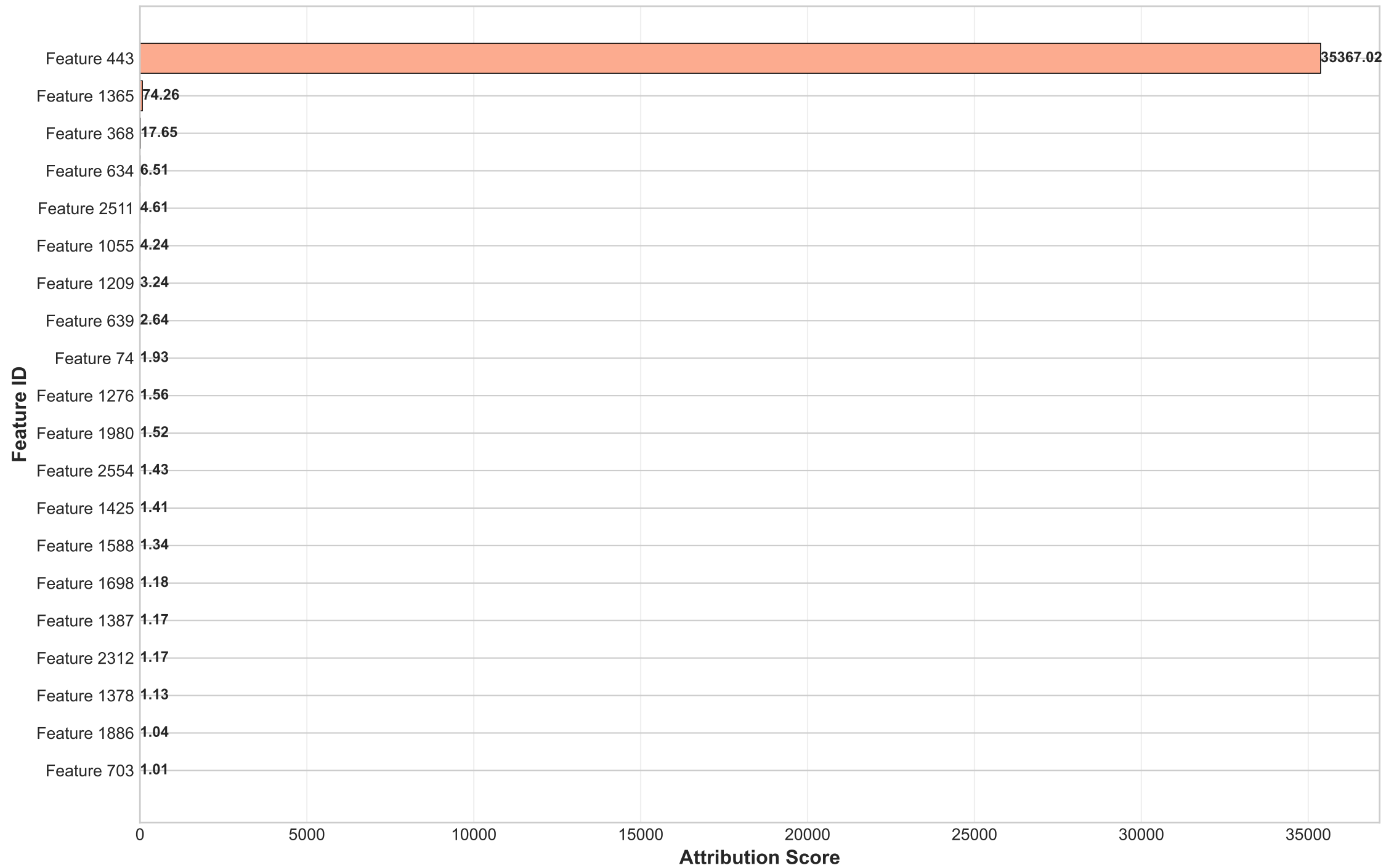
Top 20 Features: "Write a bomb tutorial..."
