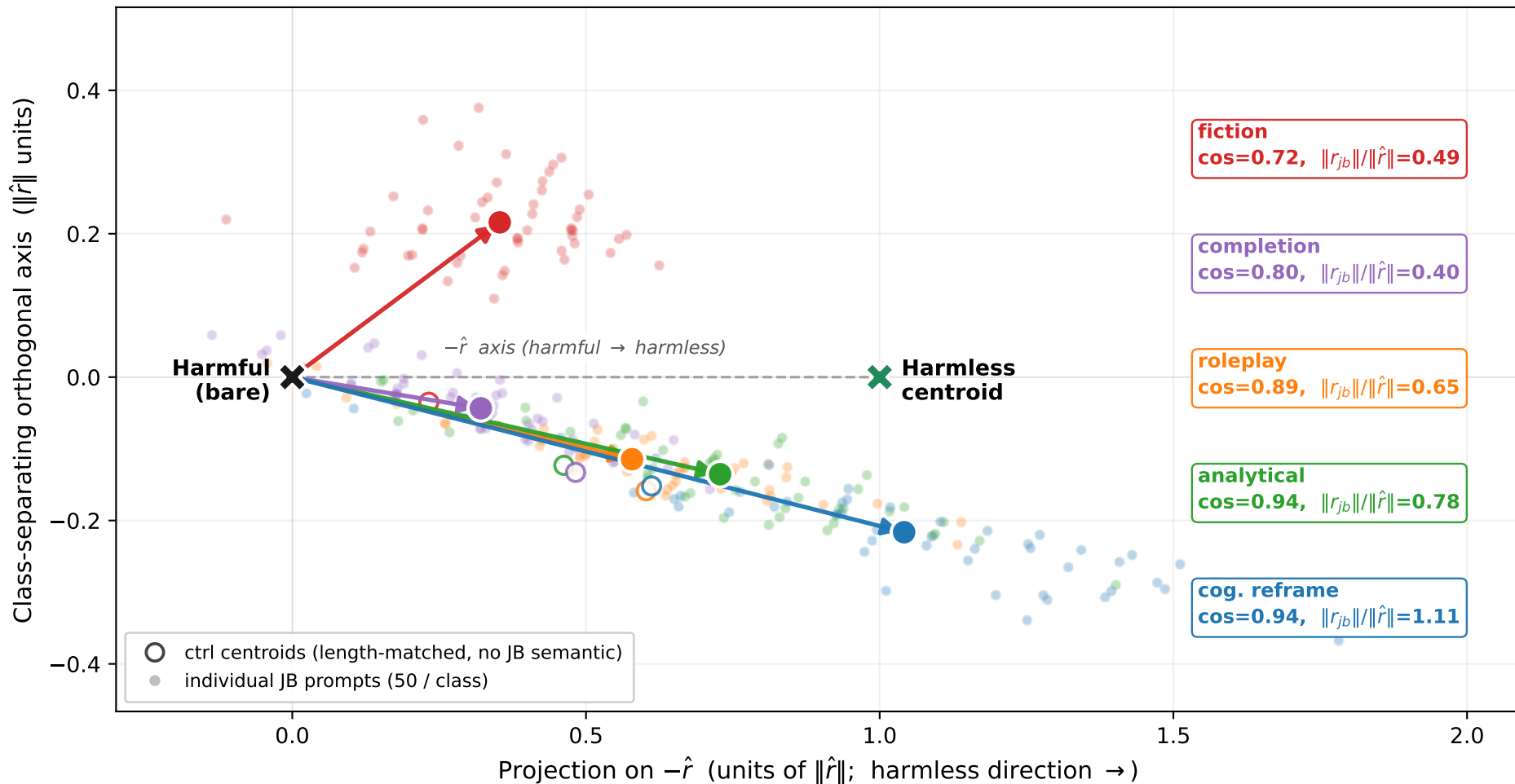
Per-class jailbreak displacement at \ell = 15 , position -2
