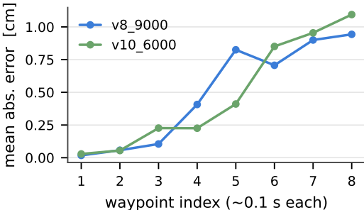
lateral error vs horizon
