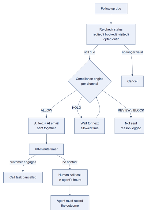
Figure 2 · What happens at every follow-up touch, in every workflow
