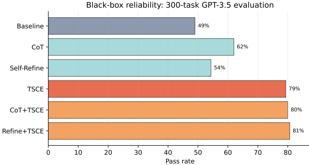
Figure 2: Outcome-level pass rates for the 300-task GPT-3.5 evaluation.
