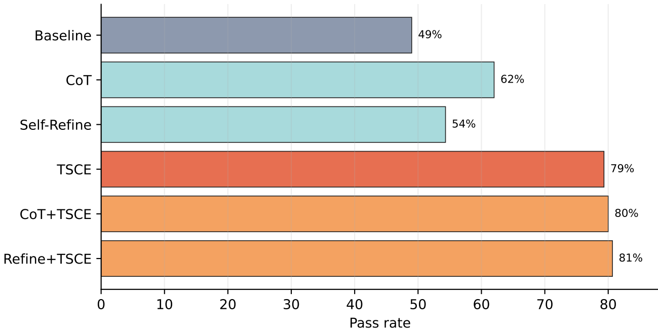
Black-box reliability: 300-task GPT-3.5 evaluation
