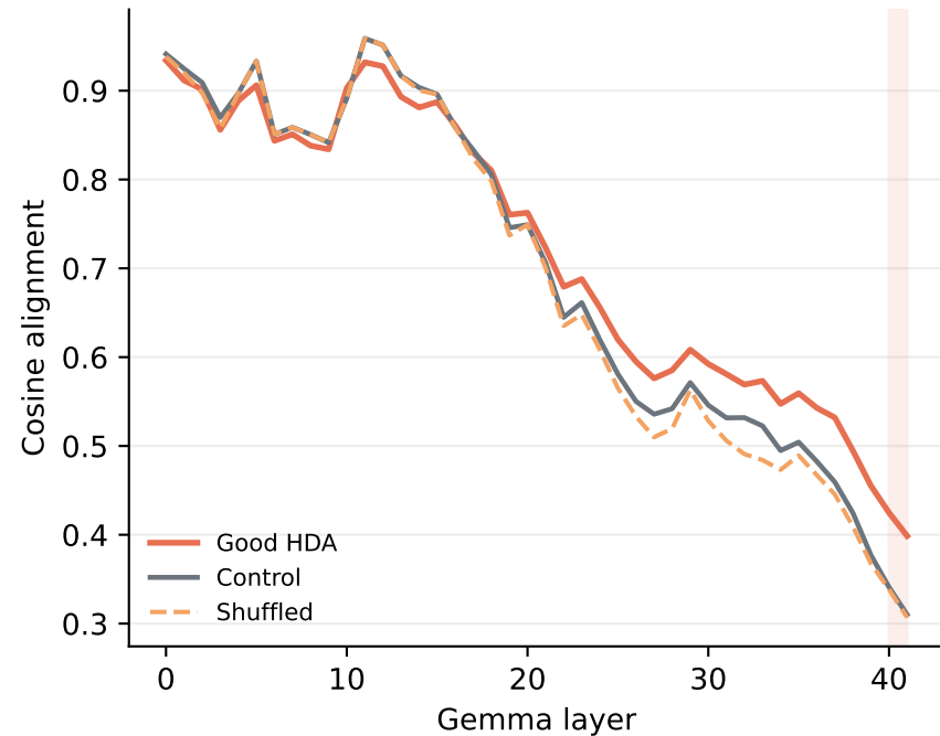
Hidden-state class alignment
