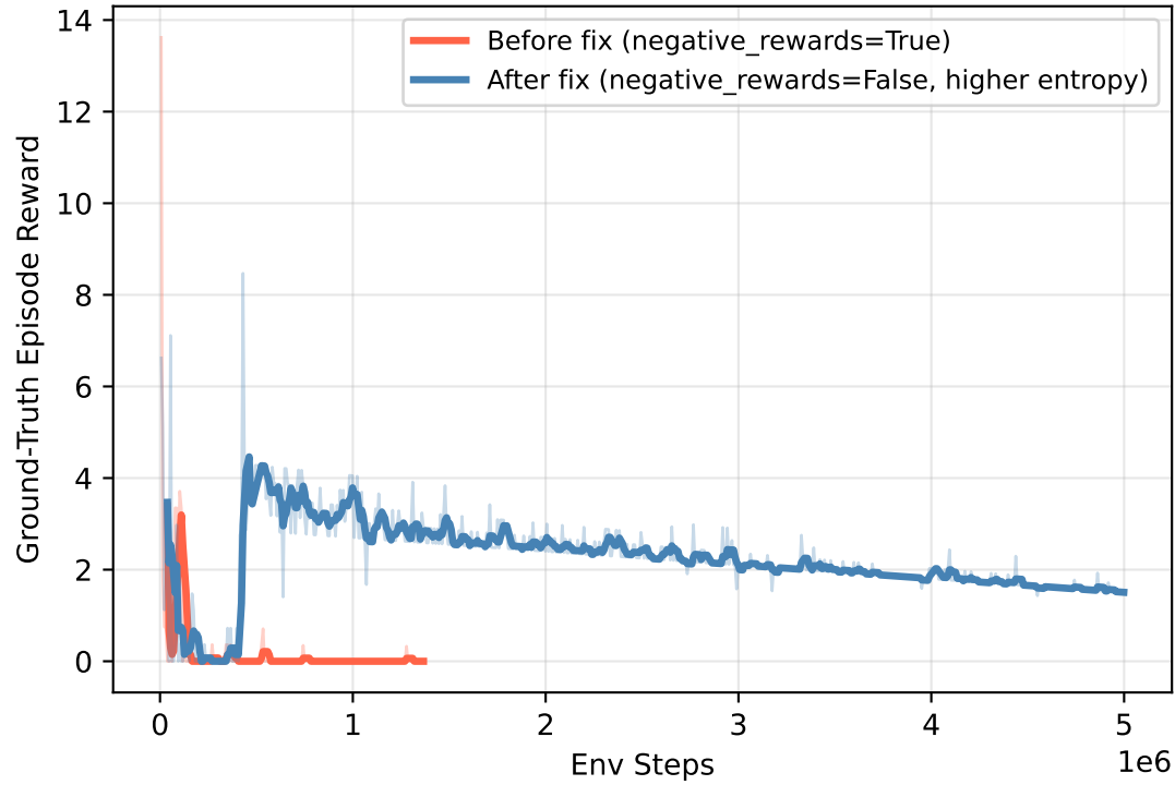
Training: Ground-Truth Reward
