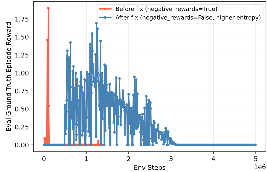
Evaluation: Ground-Truth Reward
