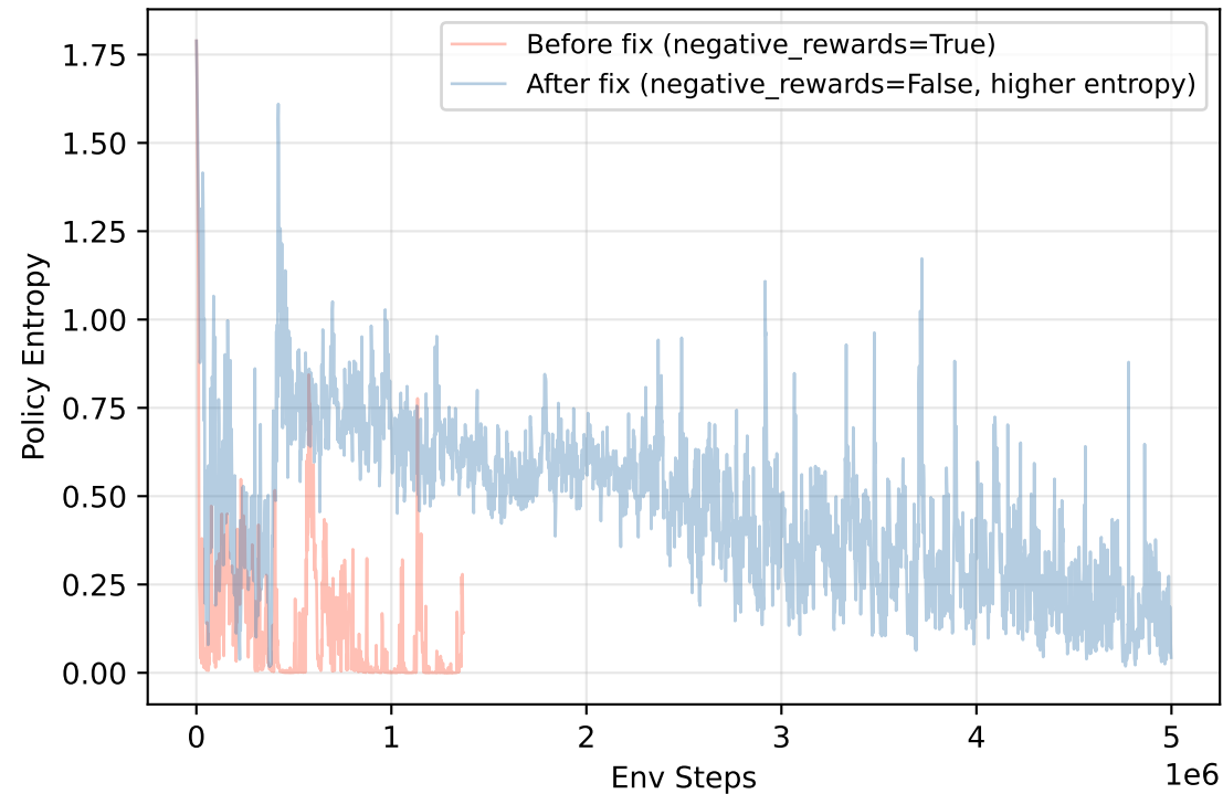
Policy Entropy (exploration vs. collapse)
