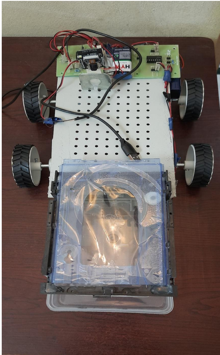
Fig 1: Final Design of Pet Food Feeder
