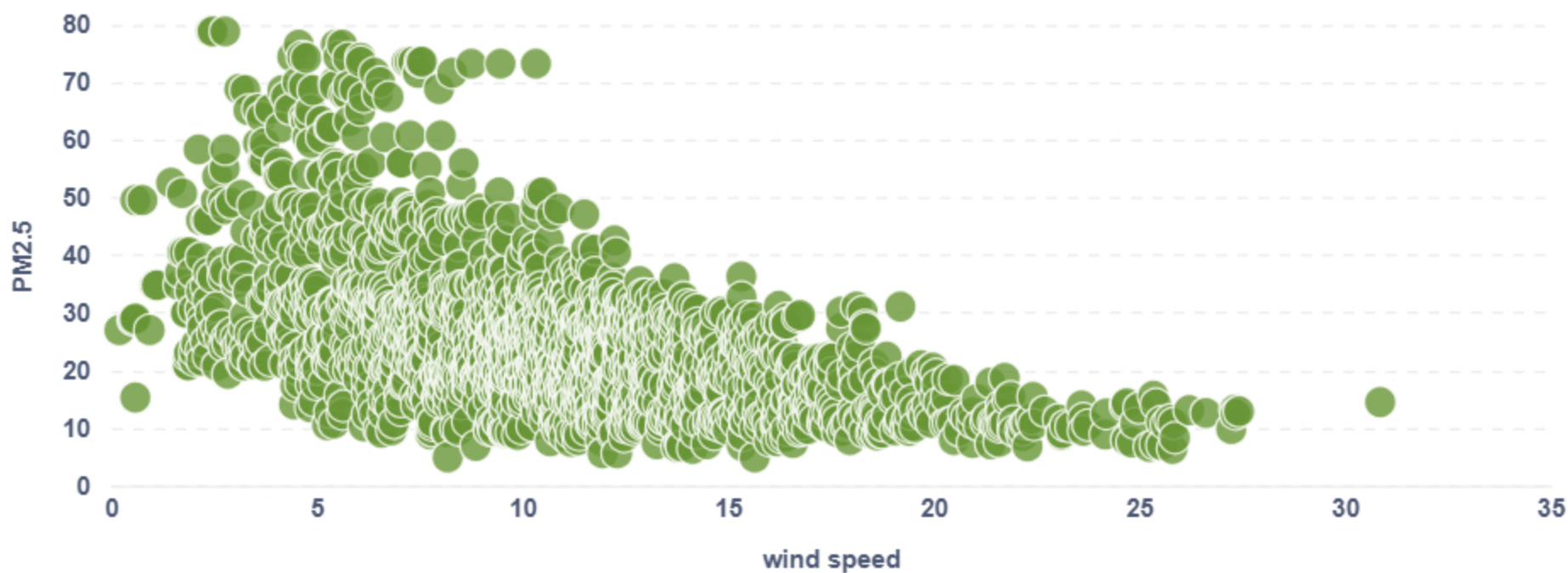
Wind Speed vs PM2.5
