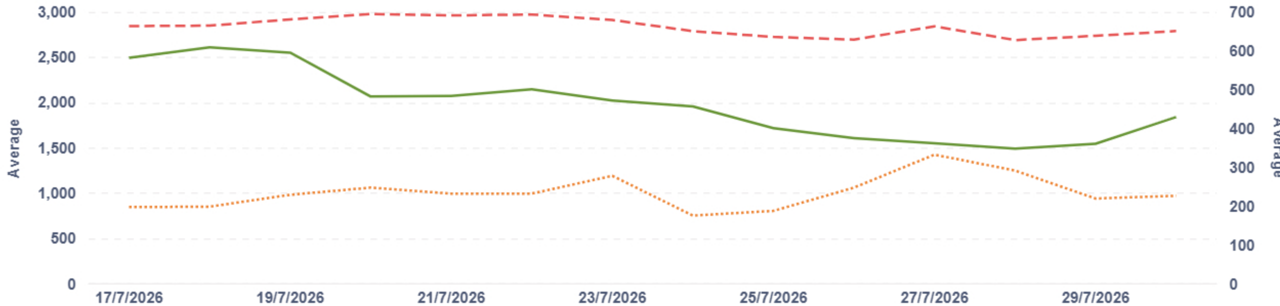
Wind Speed vs PM2.5
