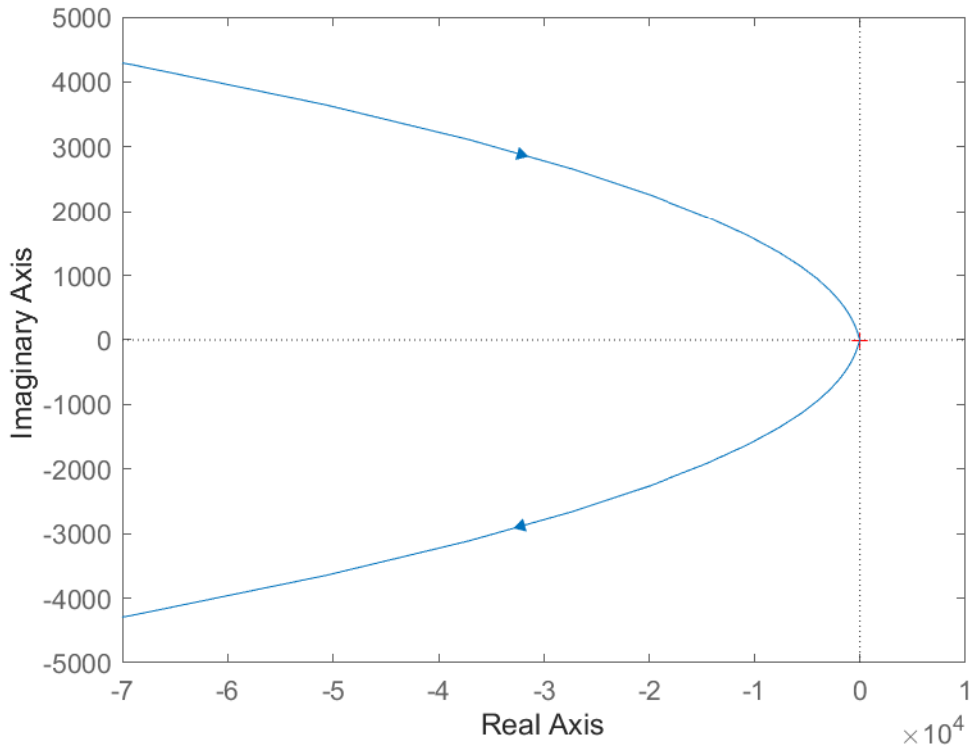
Nyquist Diagram
