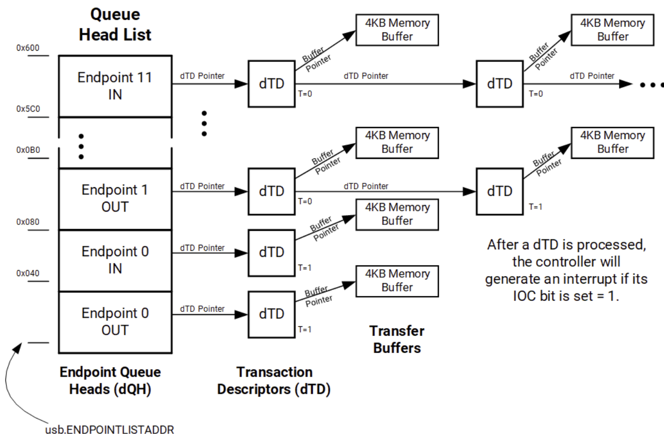
Figure: USB Device Link-list Endpoints Example
