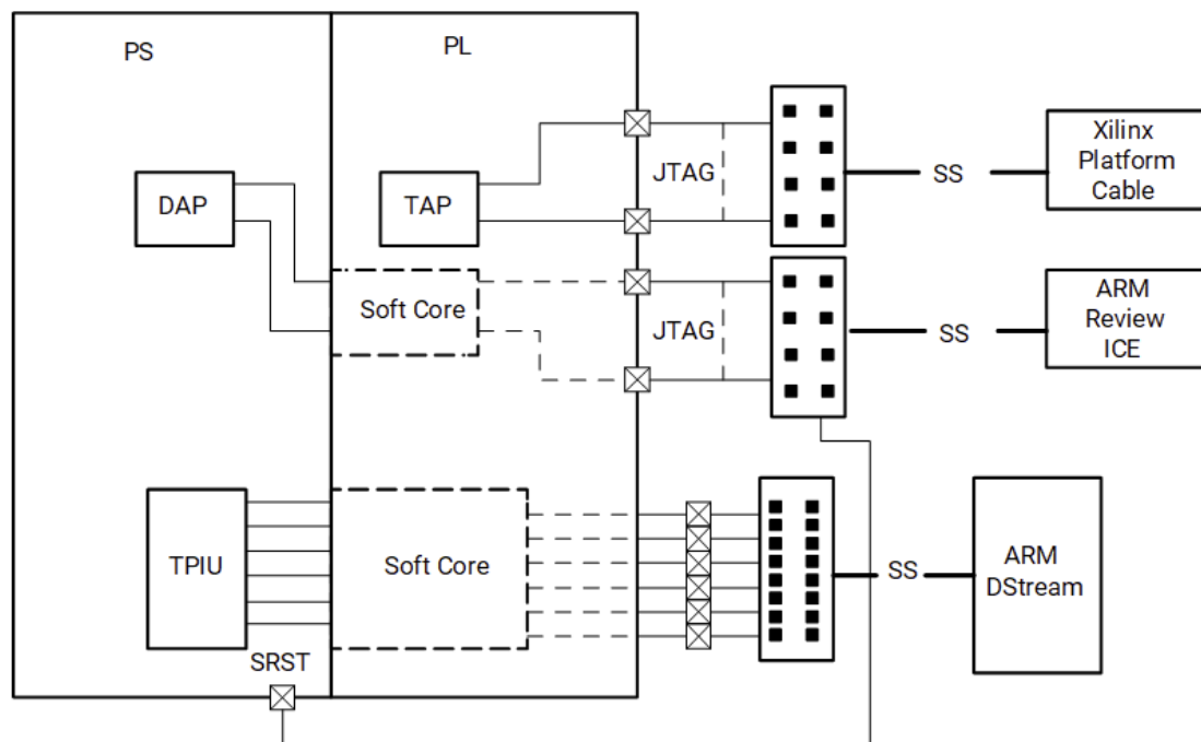
Figure: User Case II: PS and PL Debug with Trace Port Enabled
