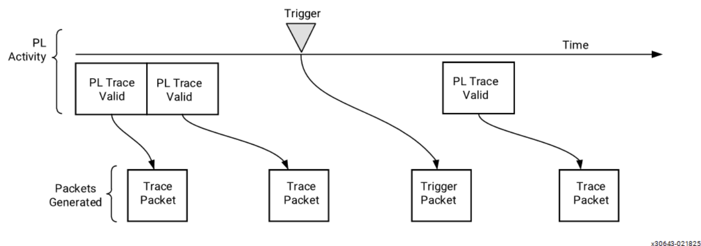
Figure: Packet Generation, No Cycle Count Case
