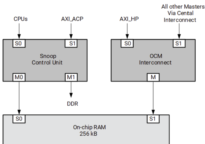
Figure: OCM System Viewpoint
