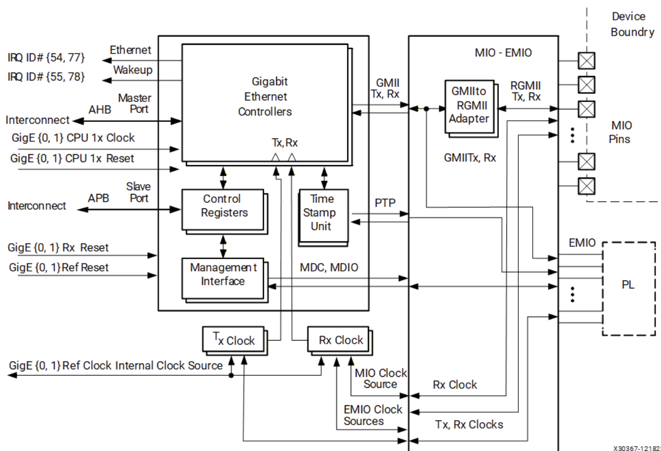
Figure: System Viewpoint
