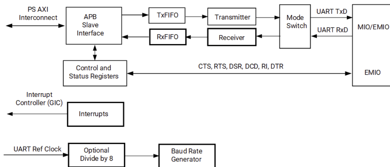
Figure: UART Block Diagram
