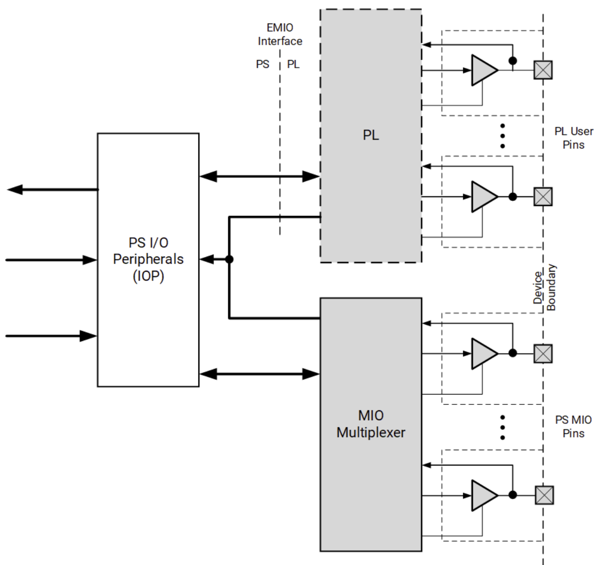
Figure: MIO-EMIO Overview
