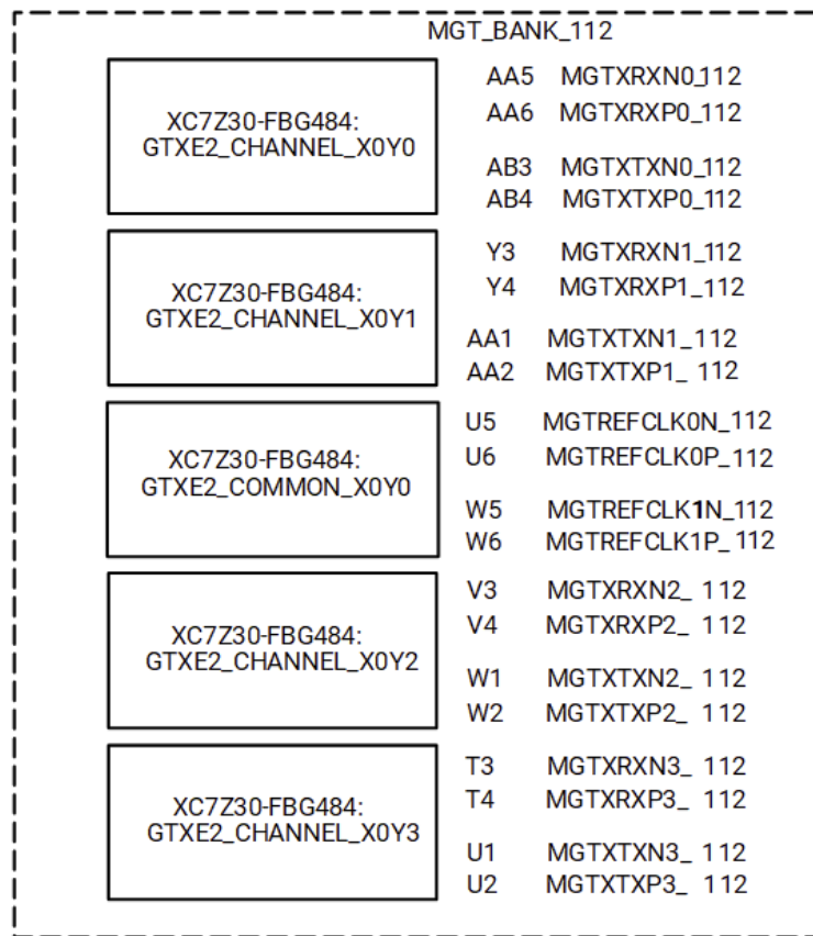
Figure: XC7Z30-FBG484 Package Placement Diagram
