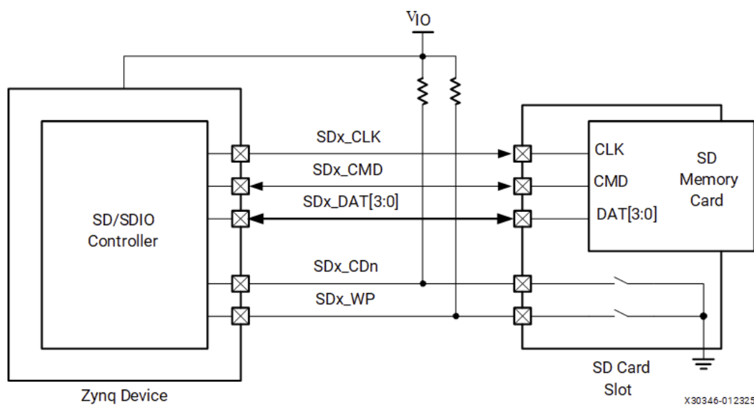
Figure: SDIO Controller SD Card Detect and Write Protect Diagram
