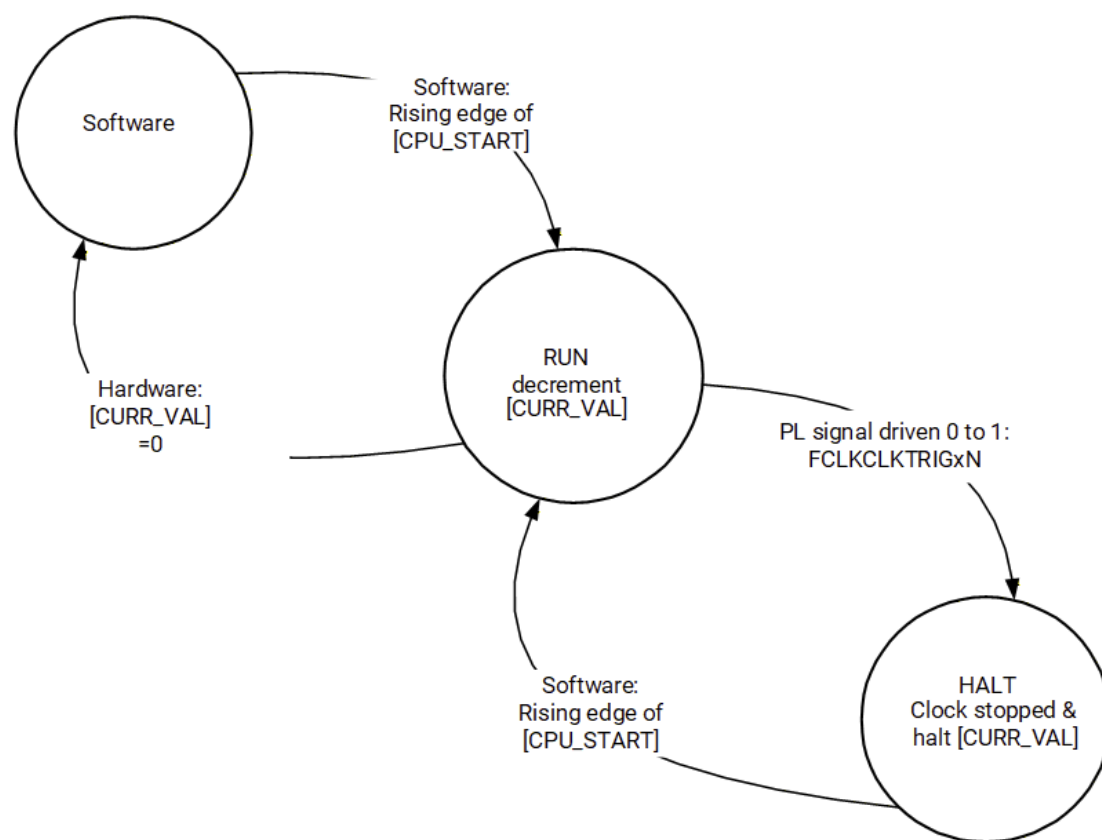
Figure: PL Clock Throttle States
