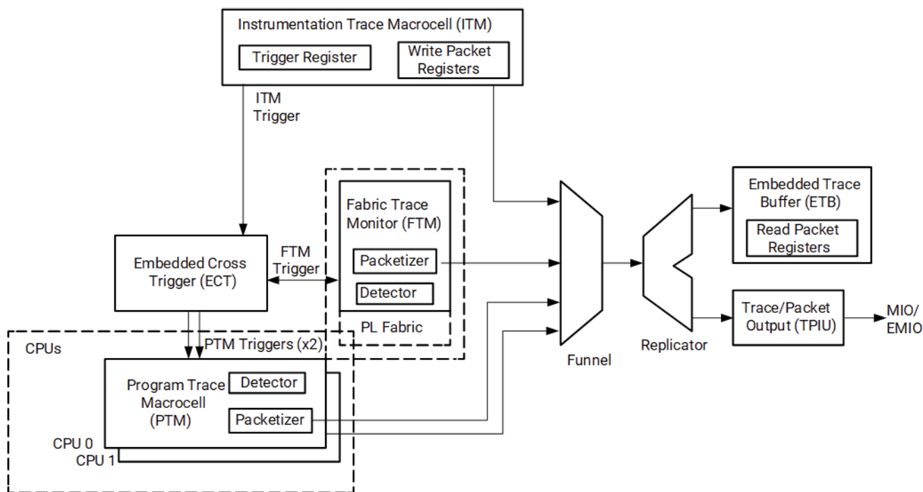
Figure: CoreSight System Block Diagram
