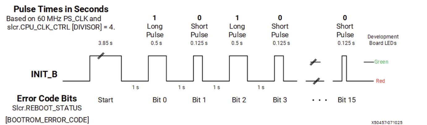
Figure: Error Code INIT_B Bit Waveform Example
