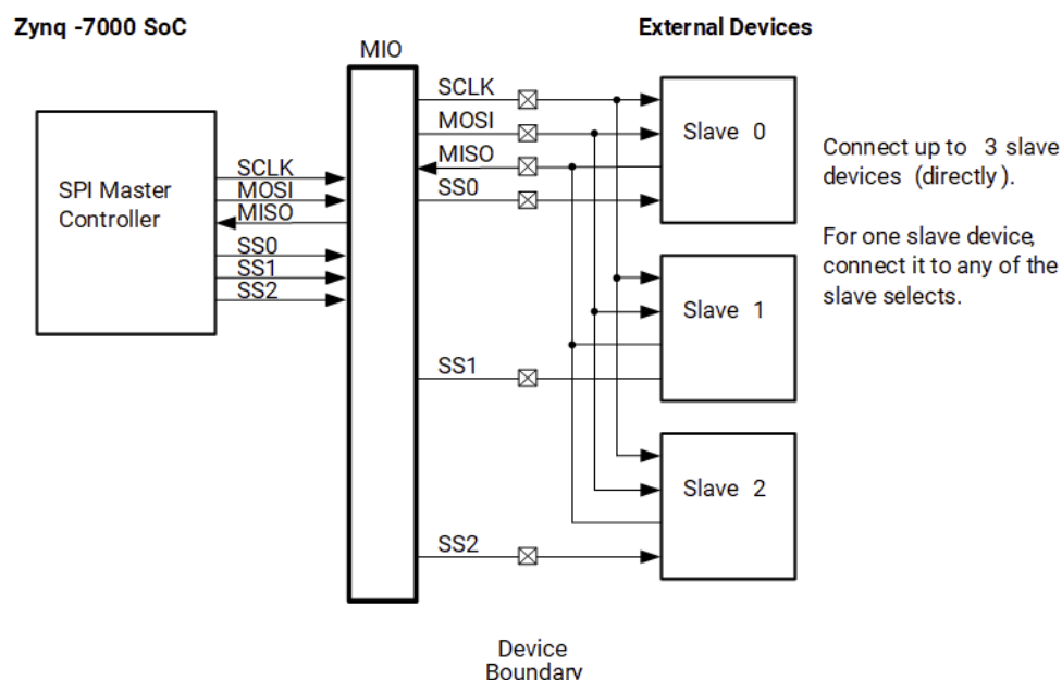
Figure: SPI Master Mode Wiring Diagram via MIO
