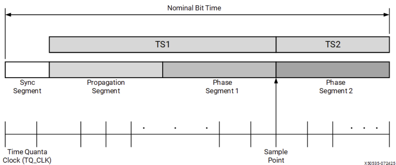
Figure: CAN Bit Time
