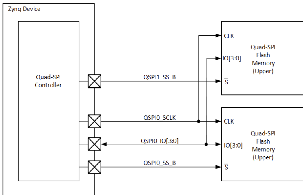
Figure: Quad-SPI Dual SS 4-bit Stacked I/O
