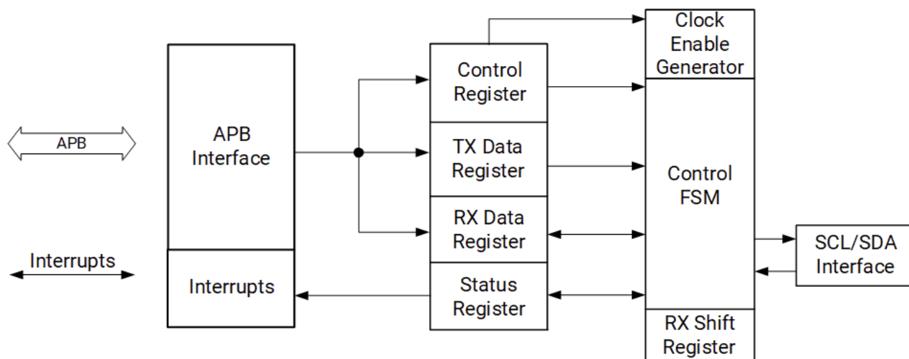
Figure: I2C Peripheral Block Diagram
