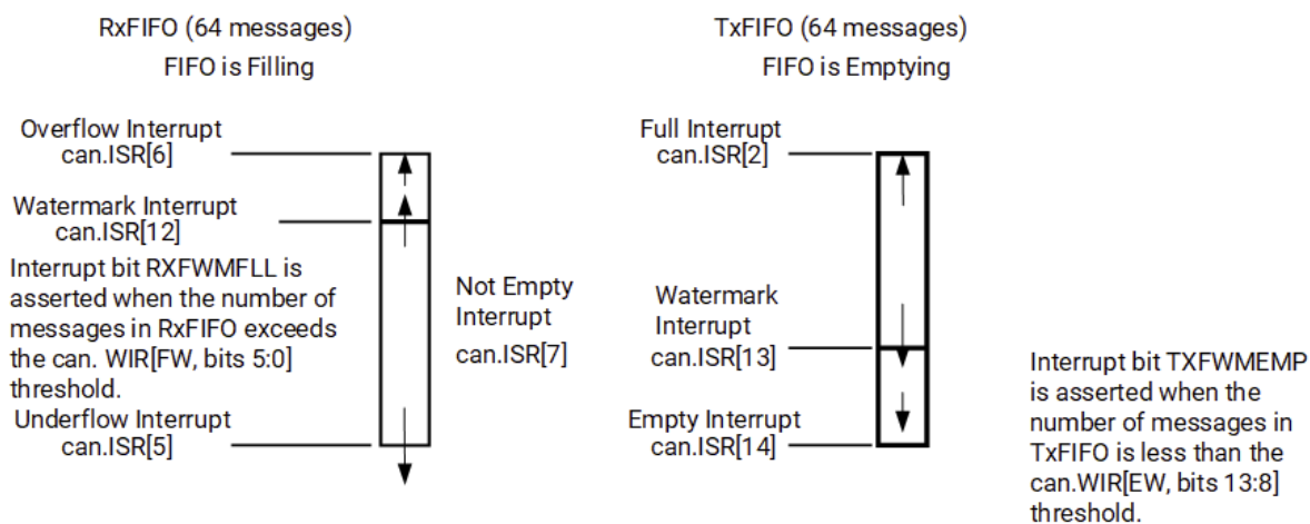
Figure: CAN RxFIFO and TxFIFO Watermark Interrupts
