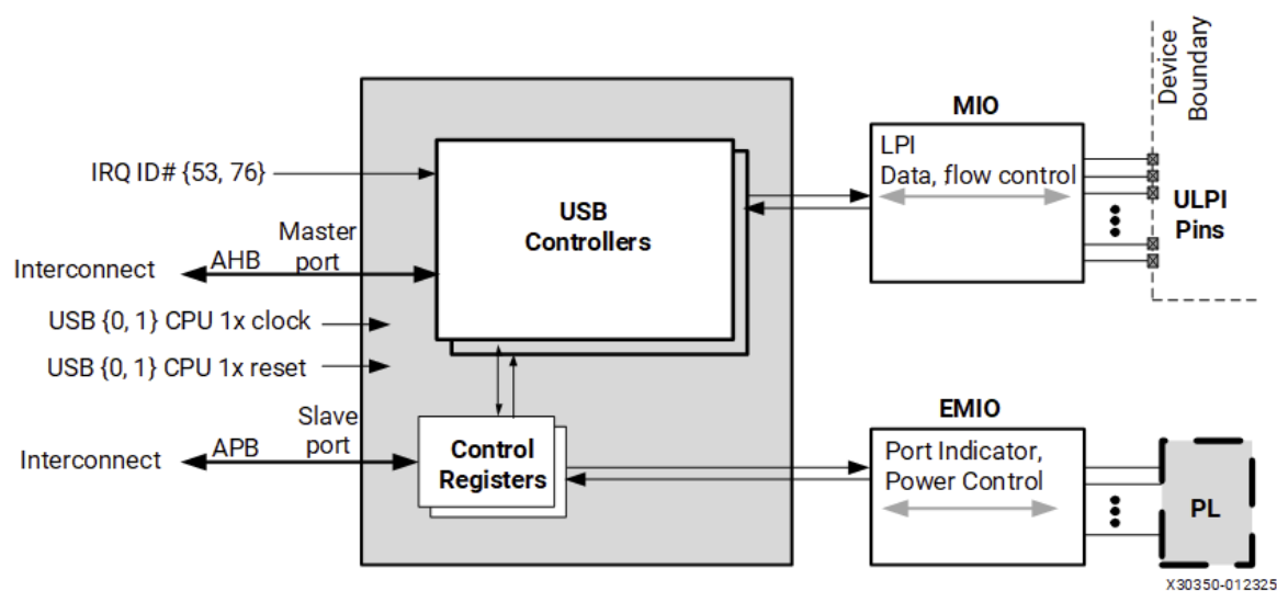
Figure: USB Hardware System Block Diagram
