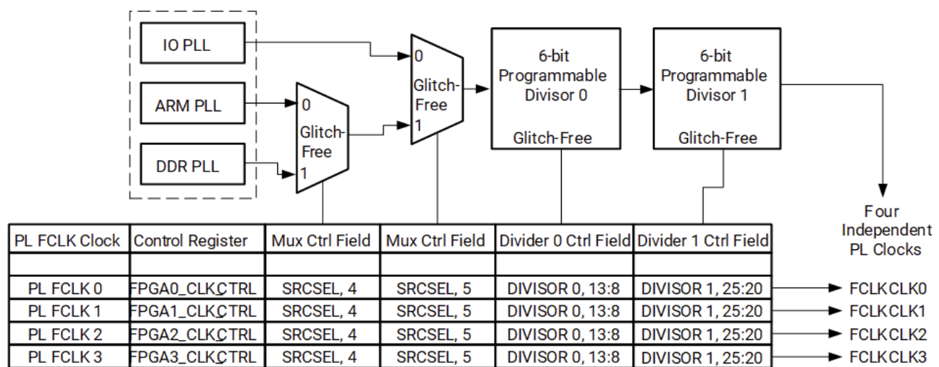
Figure: PL Clock Generation
