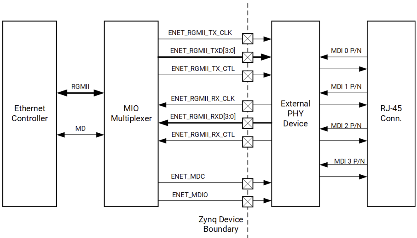
Figure: Ethernet Communications Wiring Connections
