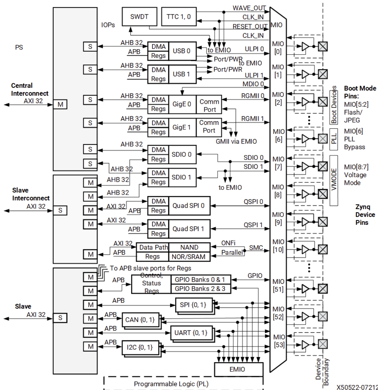
Figure: I/O Peripherals System Diagram
