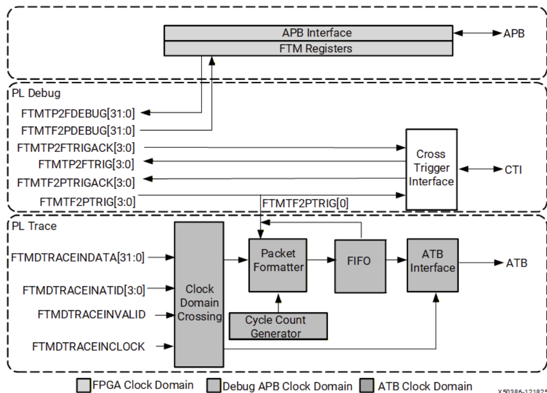
Figure: FTM Block Diagram
