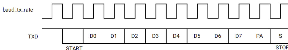
Figure: Transmitted Data Stream
