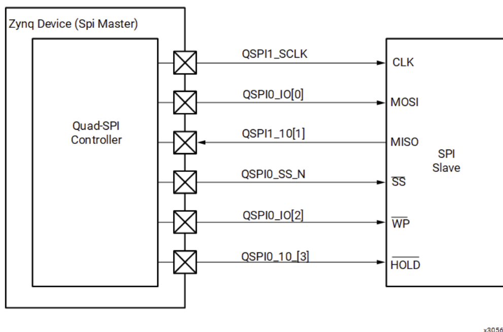
Figure: Quad-SPI Single SS, Legacy I/O
