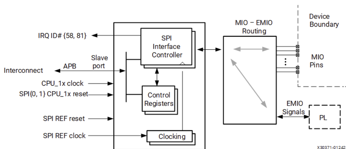
Figure: SPI System Block Diagram
