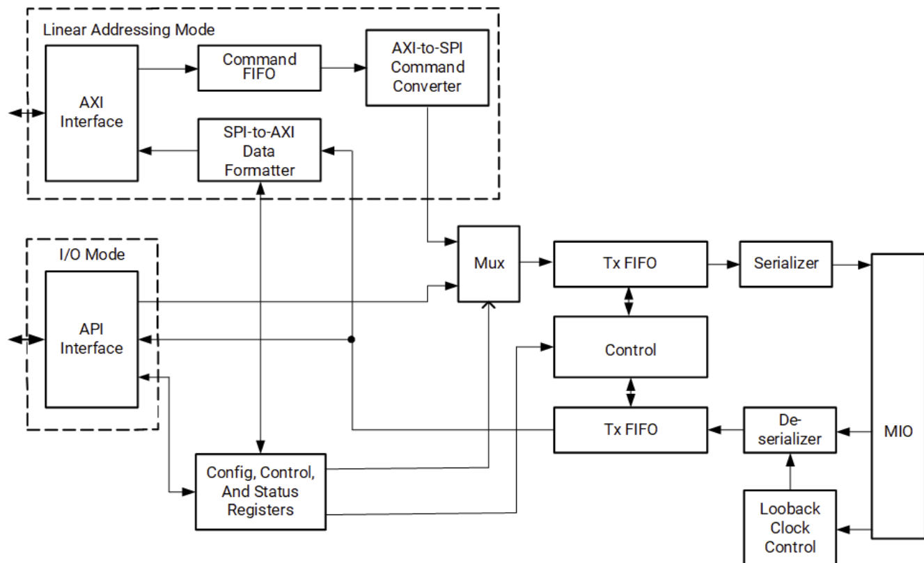
Figure: Quad-SPI Controller Block Diagram
