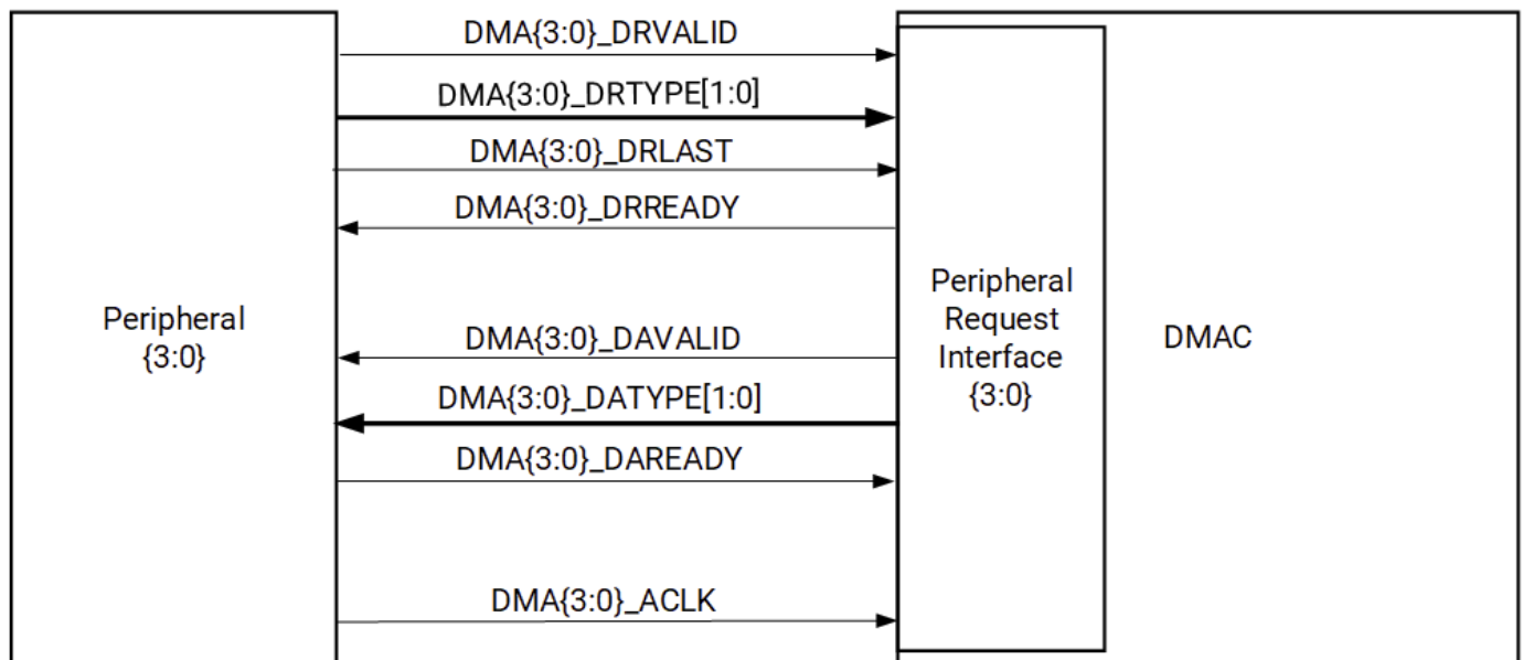
Figure: DMAC PL Peripheral Request Interface Request/Acknowledge Signals
