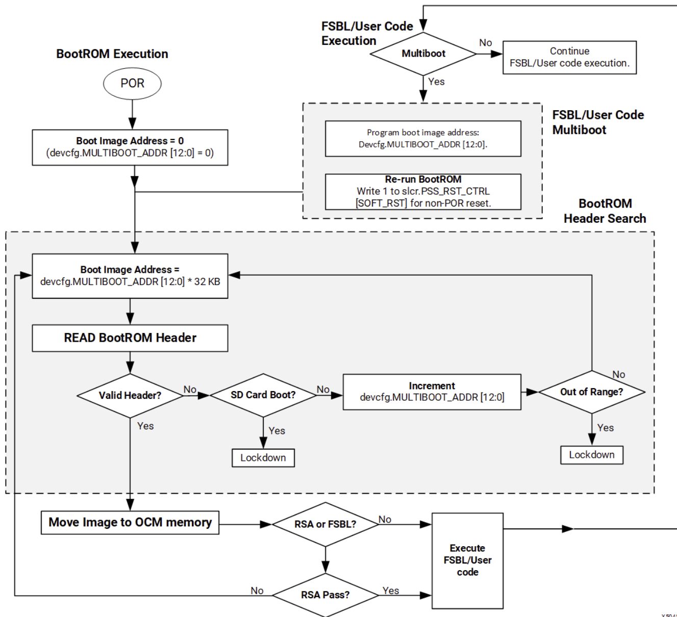
Figure: BootROM Header Search and FSBL/User Code Multiboot Flowchart
