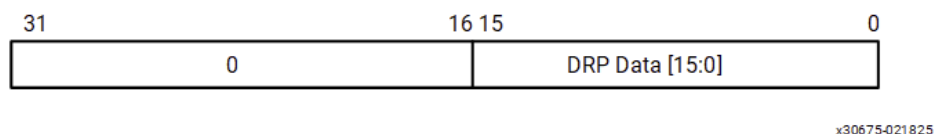
Figure: PS-XADC Interface Read Data Format
