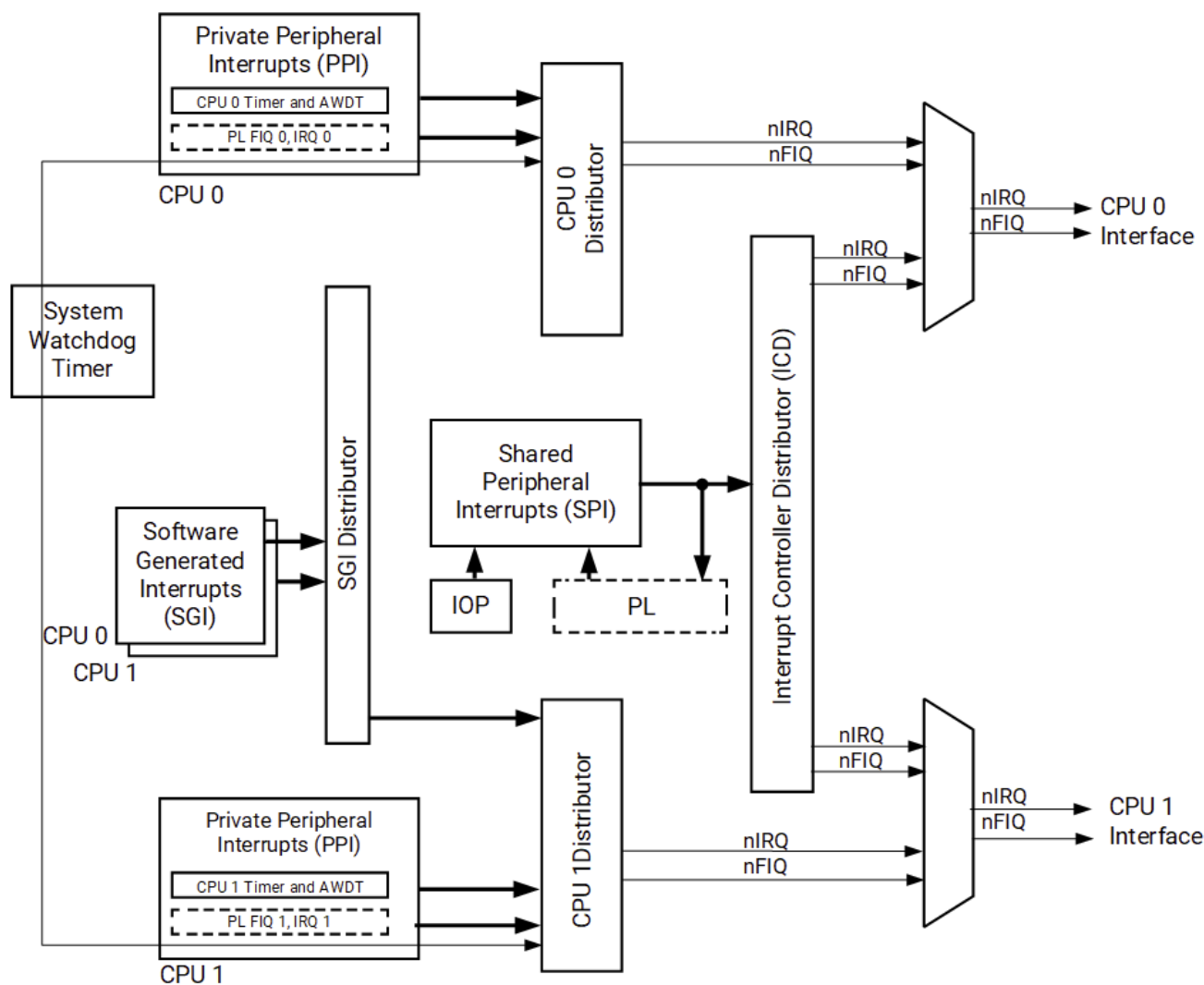
Figure: Interrupt Controller Block Diagram
