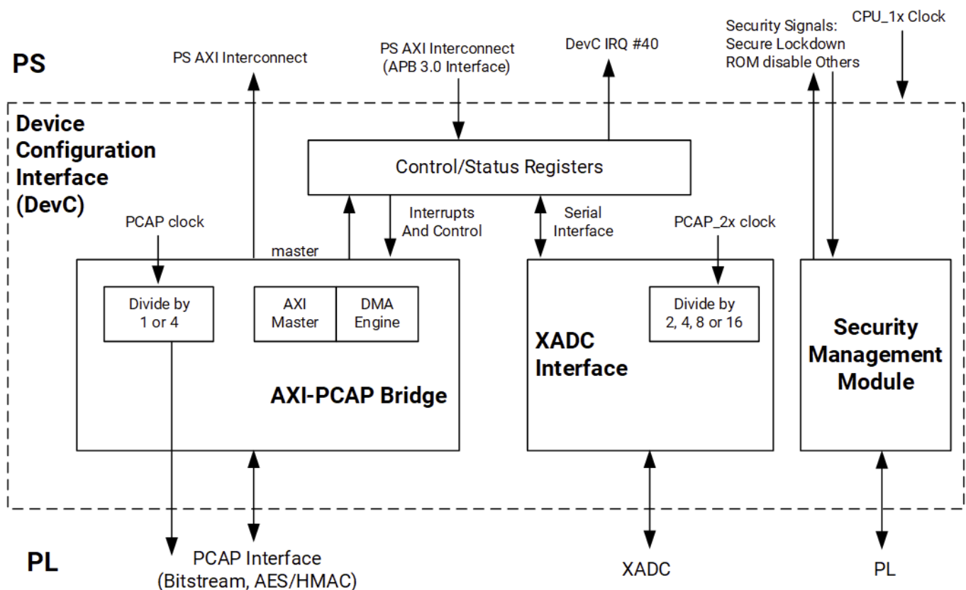
Figure: DevC Block Diagram
