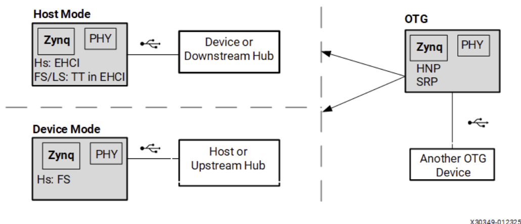
Figure: USB Controller Operating Modes
