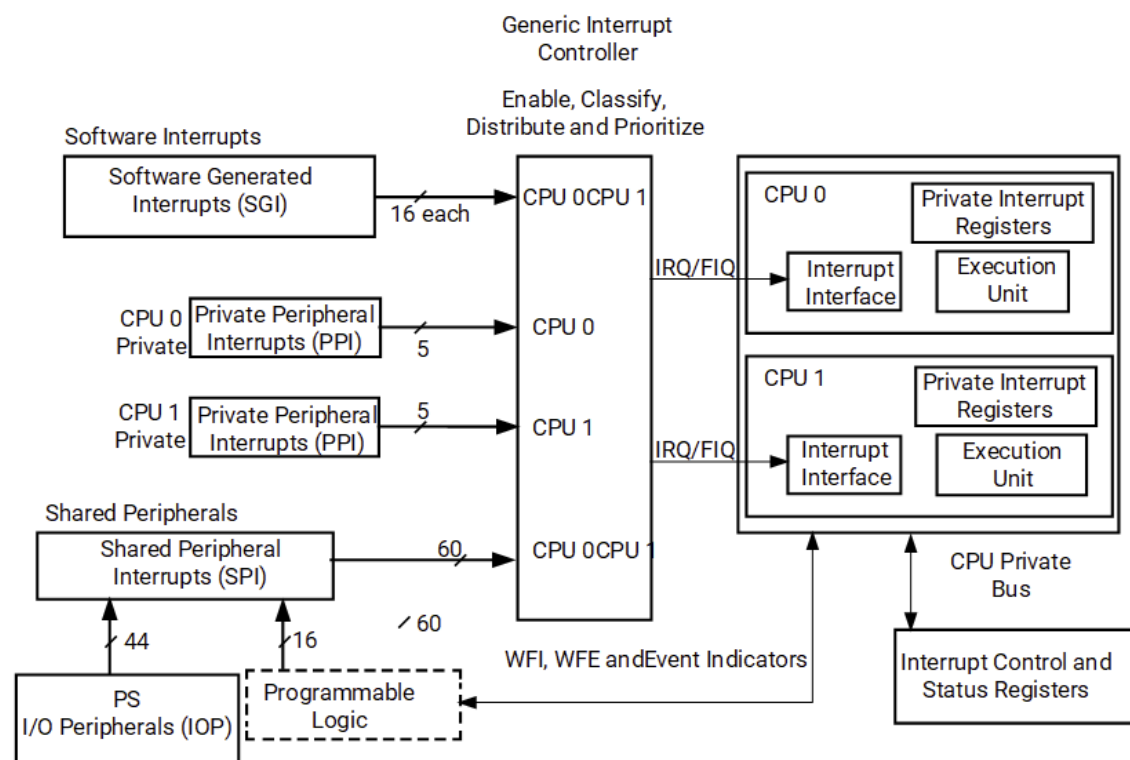
Figure: System-Level Block Diagram
