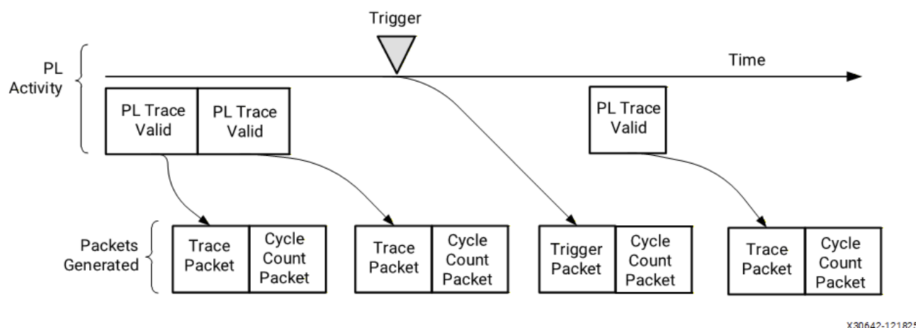
Figure: Packet Generation, Typical Case
