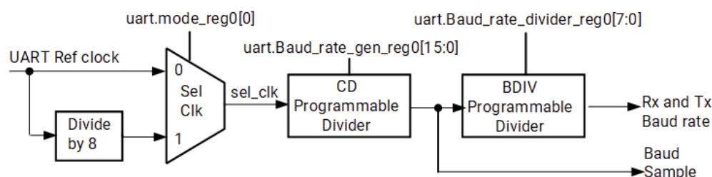
Figure: UART Board Rate Generator
