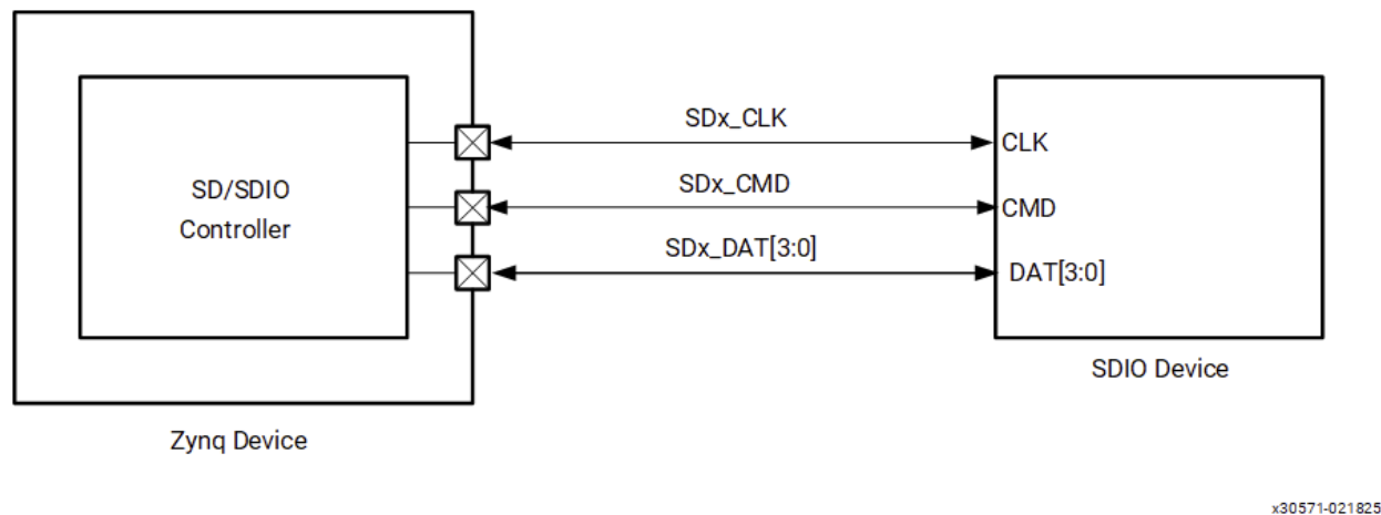
Figure: SDIO Controller Device Wiring Diagram
