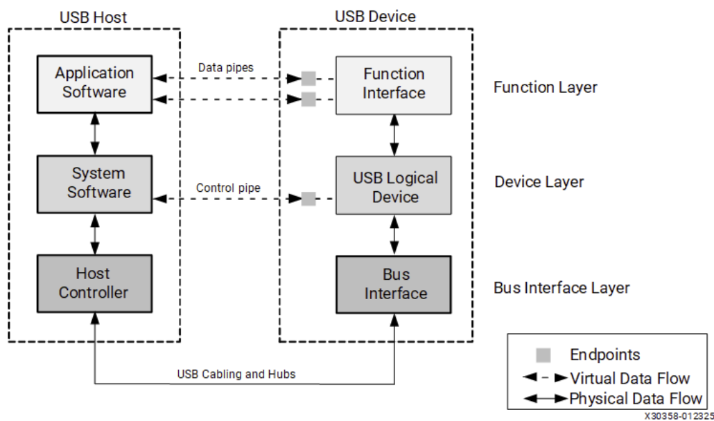
Figure: USB System Stack
