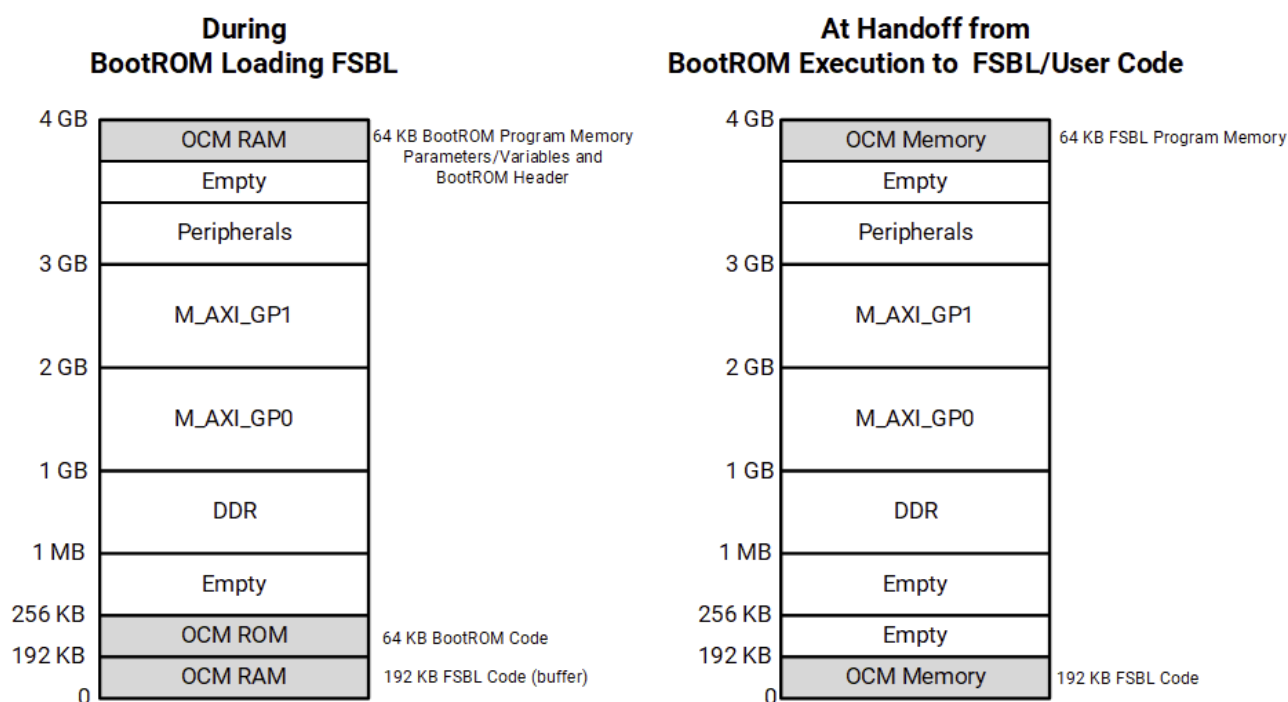
Figure: System Memory Map During BootROM Execution
