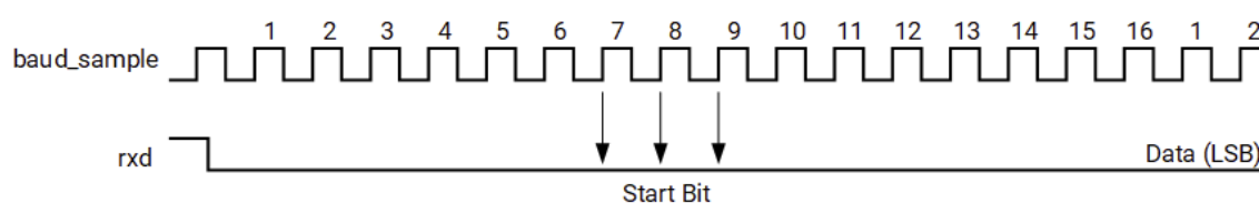
Figure: Default BDIV Receiver Data Stream
