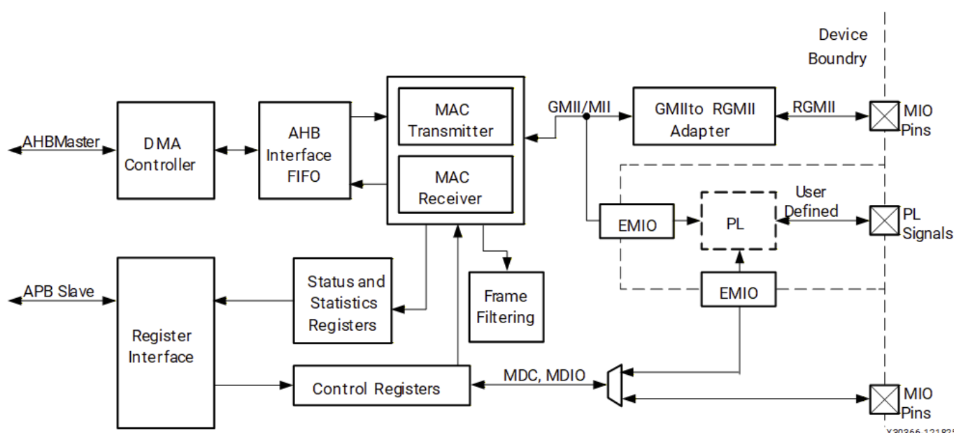
Figure: Ethernet Controller
