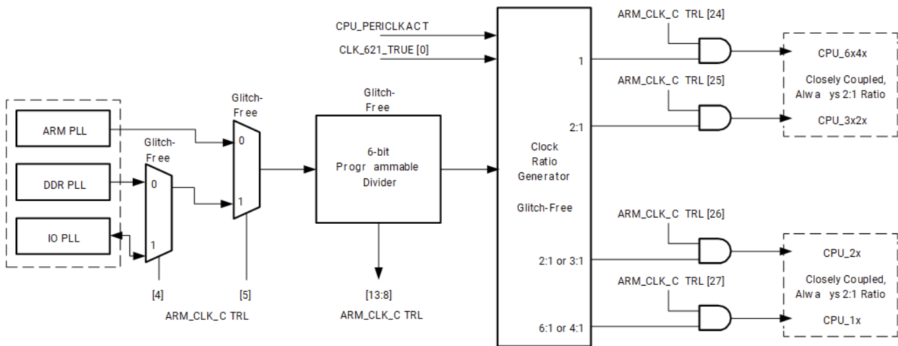
Figure: CPU Clock Generation and Domains
