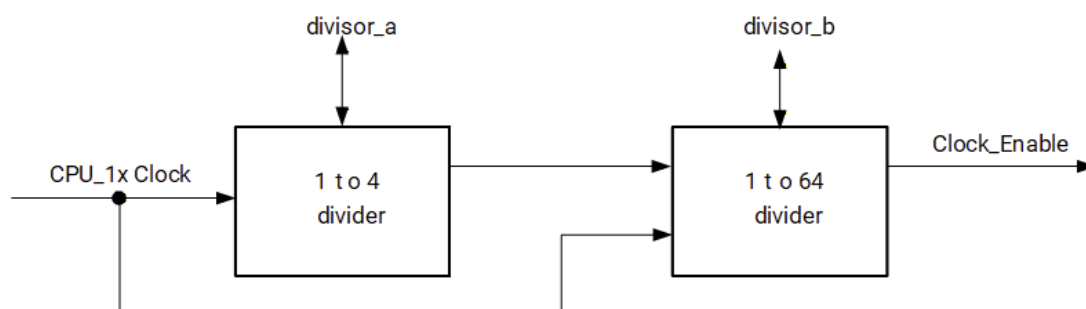
Figure: I2C Clock Generator
