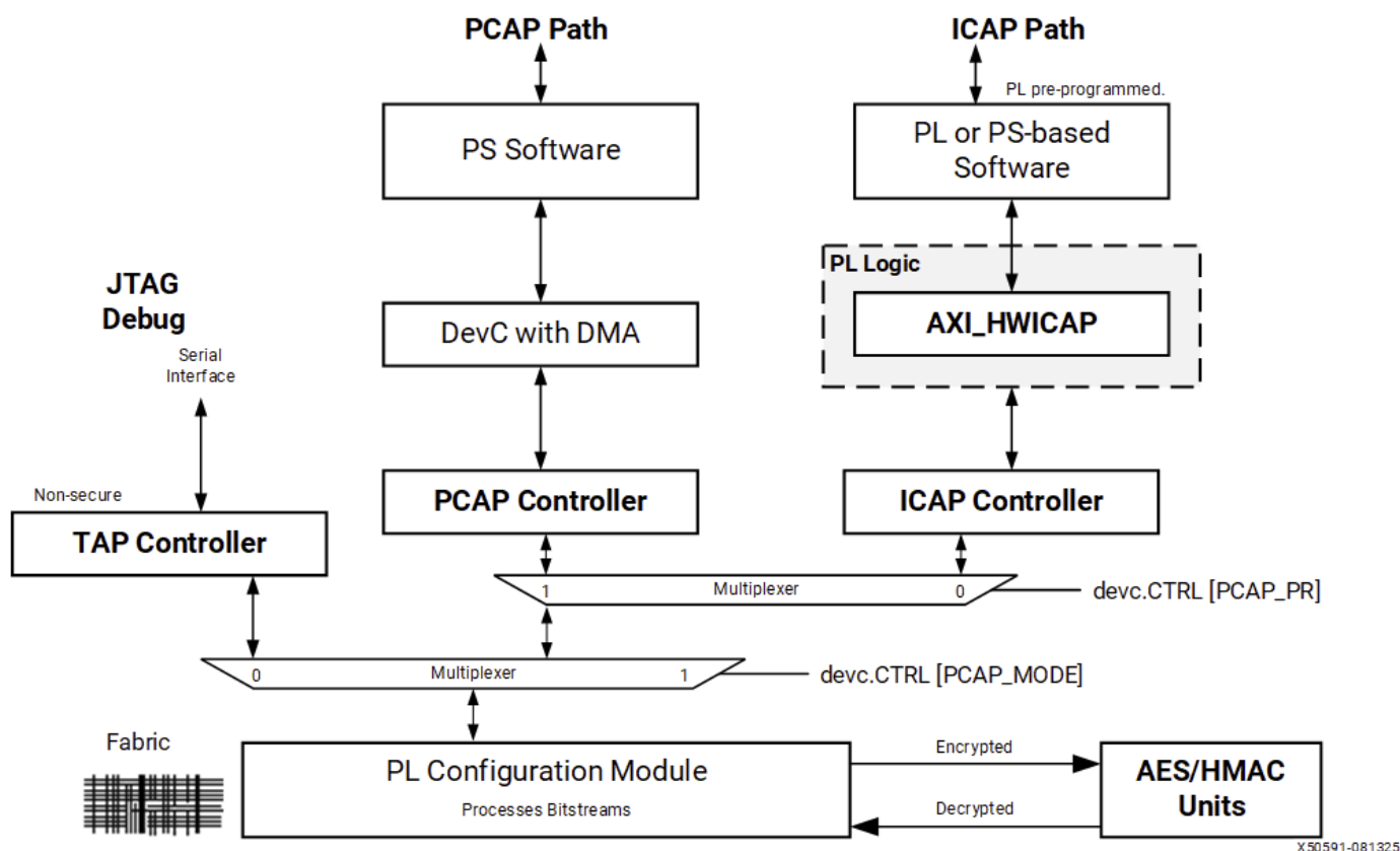
Figure: PL Configuration Paths
