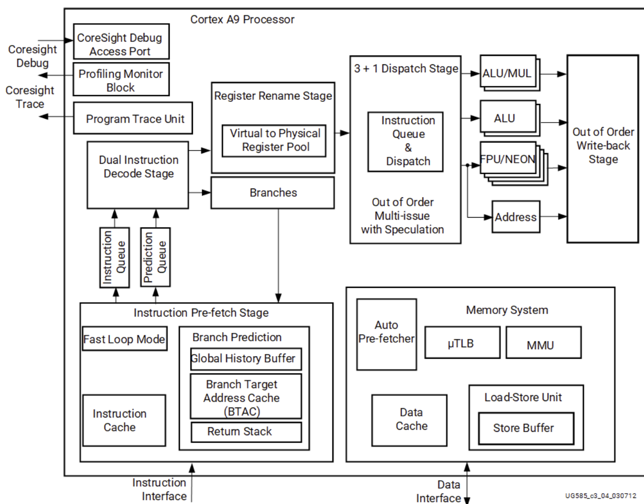
Figure: Cortex-A9 Architecture
