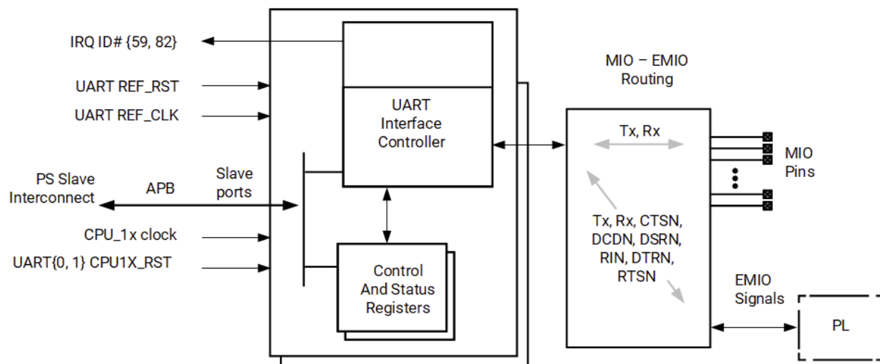
Figure: UART System Viewpoint
