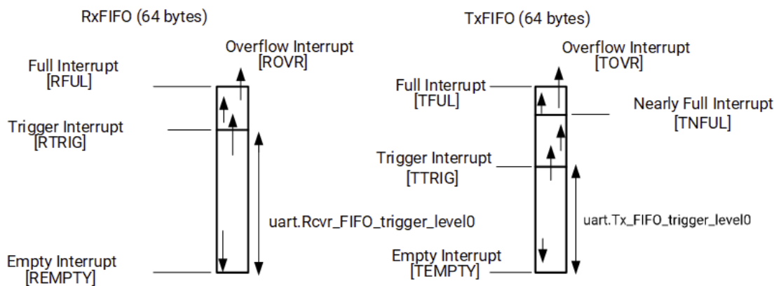
Figure: UART RxFIFO and TxFIFO Interrupt
