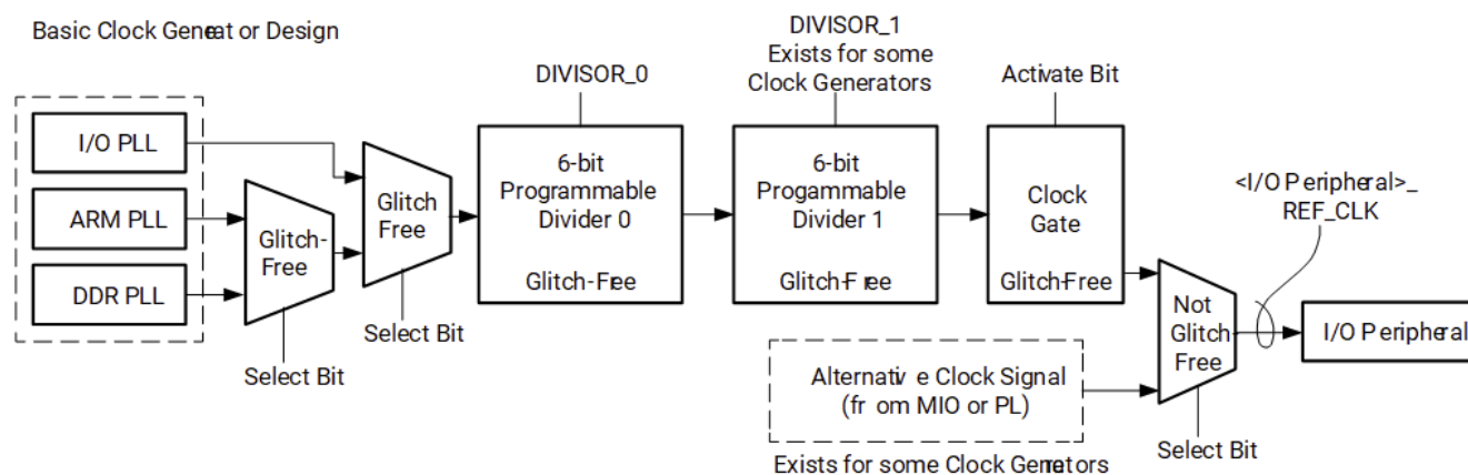
Figure: Basic Clock Branch Design
