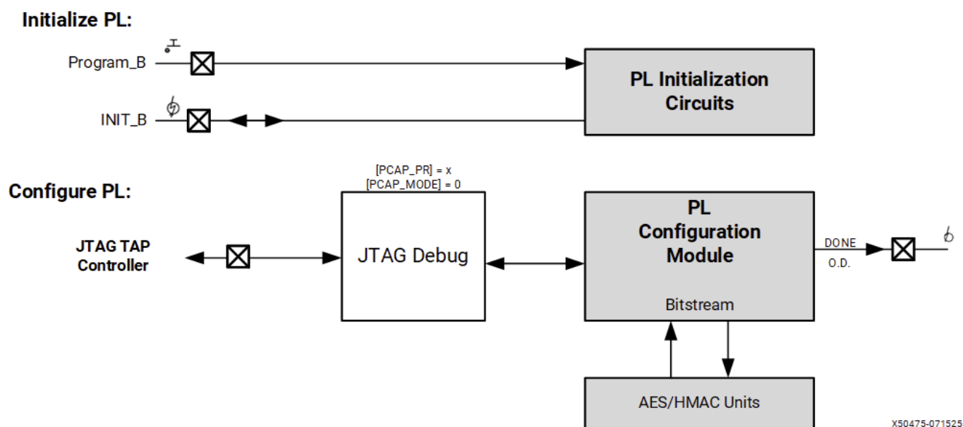
Figure: PL Initialization and Configuration Using User-JTAG
