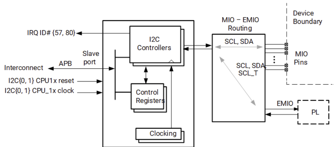
Figure: I2C System Block Diagram
