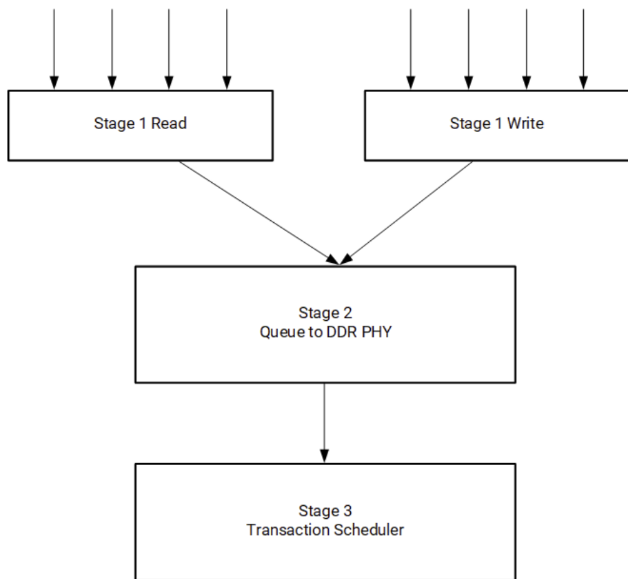
Figure: DDRC Arbitration
