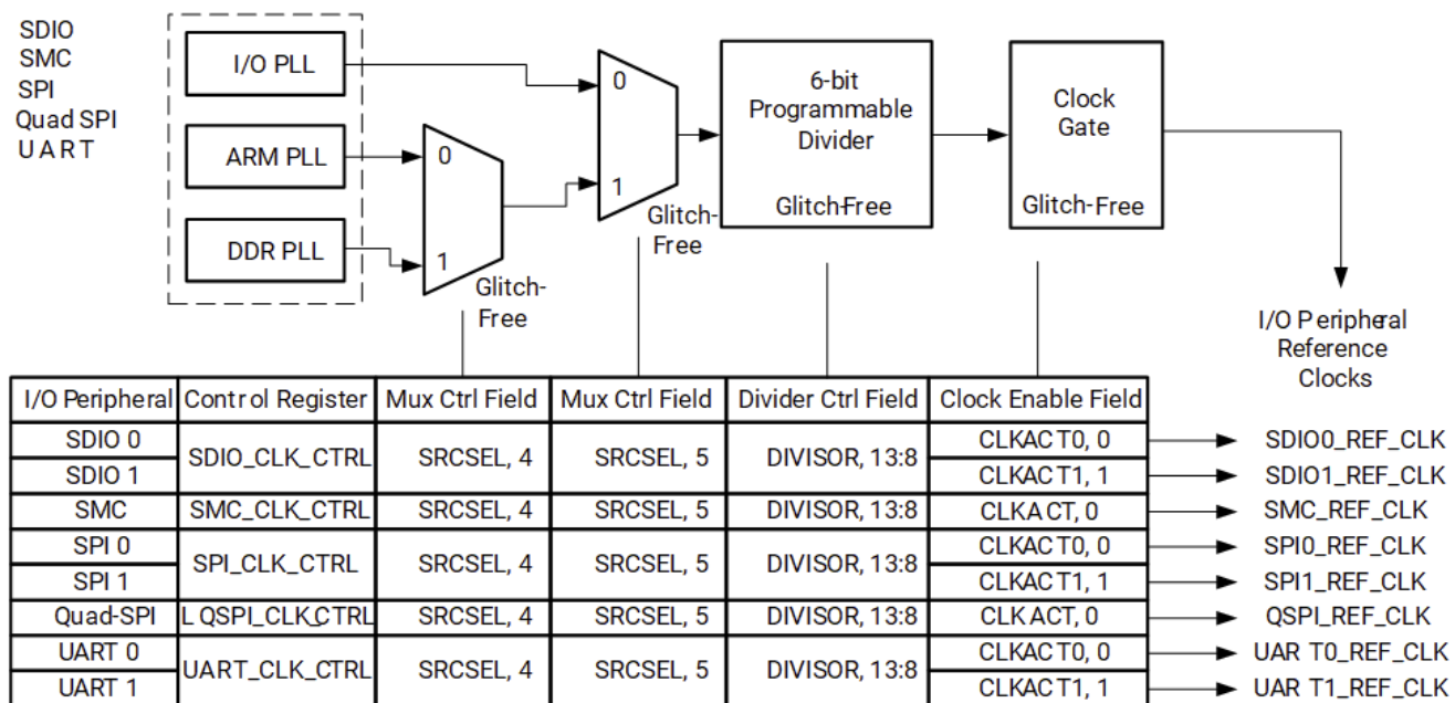
Figure: SDIO, SMC, SPI, Quad SPI and UART Reference Clocks
