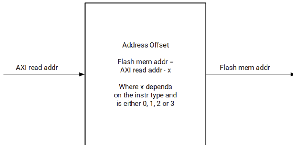
Figure: Automatic Address Offset For Word Alignment
