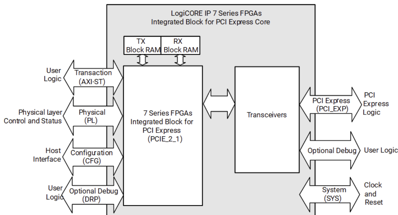
Figure: PCI Express Block Diagram
