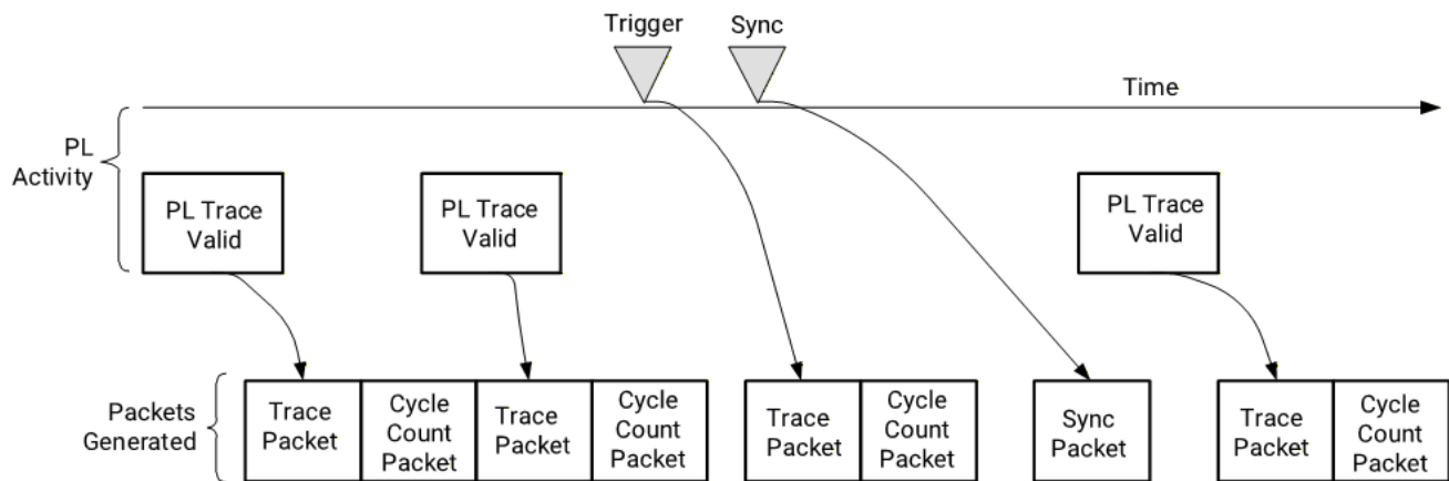
Figure: Packet Generation, Synchronization Case
