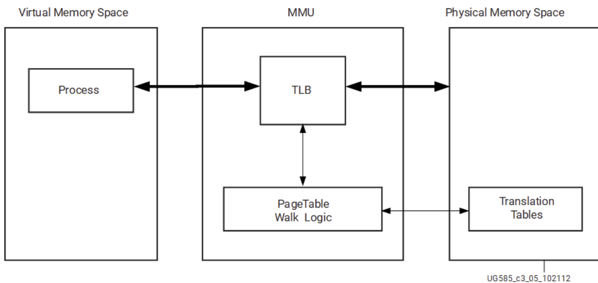
Figure: MMU Architecture Block Diagram
