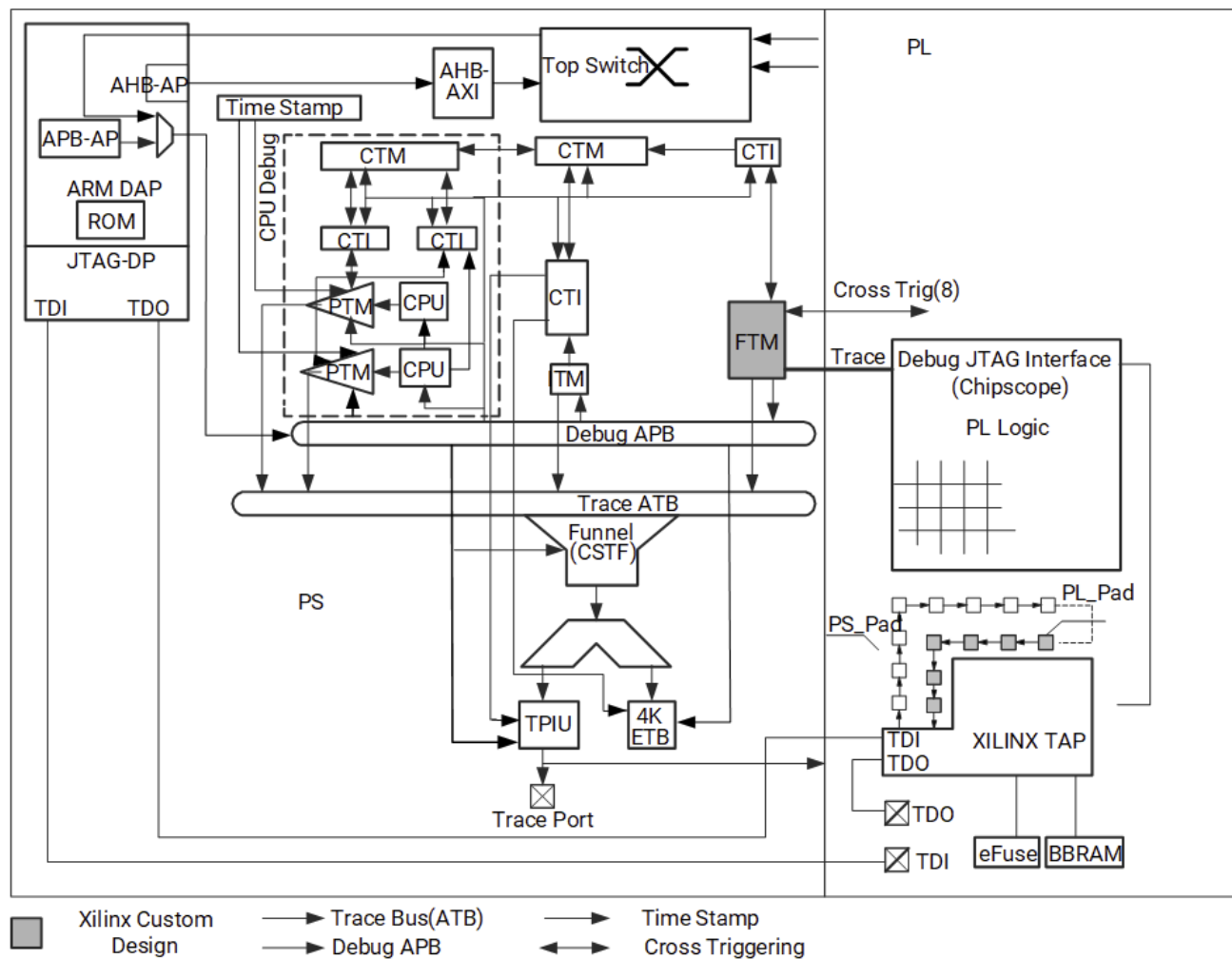
Figure: Debug System Architecture
