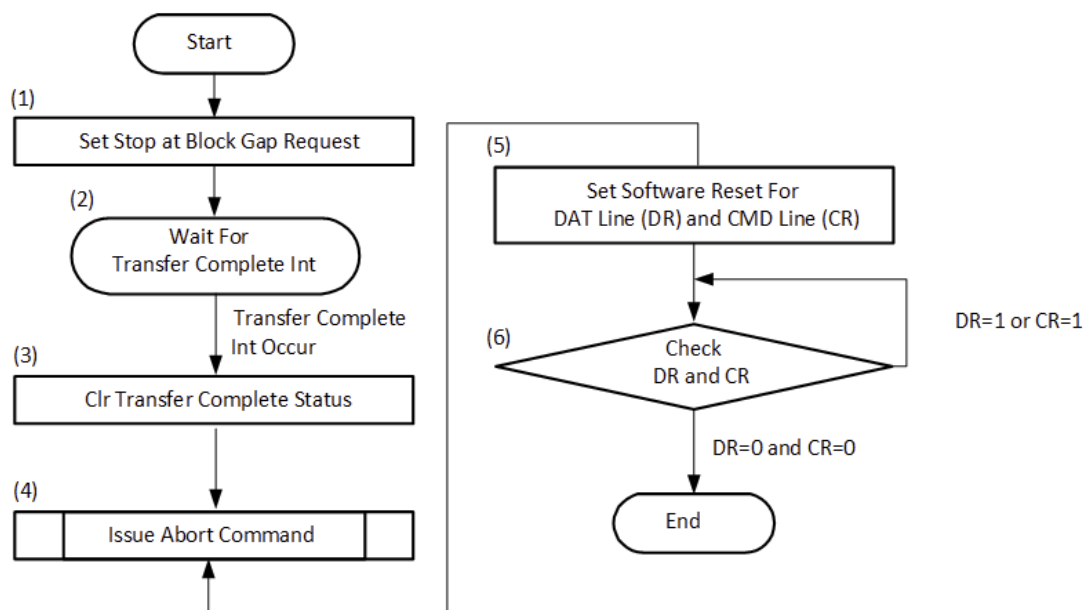
Figure: SDIO Controller Synchronous Abort Sequence
