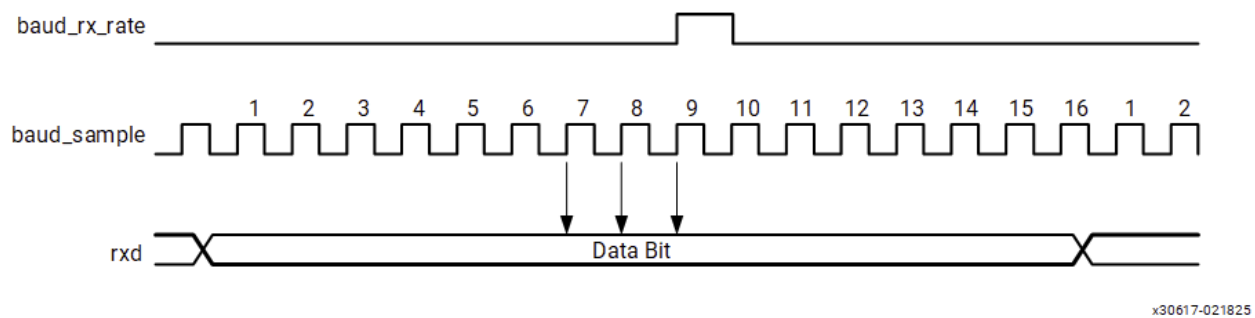
Figure: Re-synchronized Receiver Data Stream
