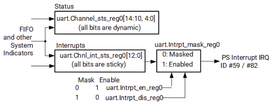
Figure: Interrupts and Status Signals
