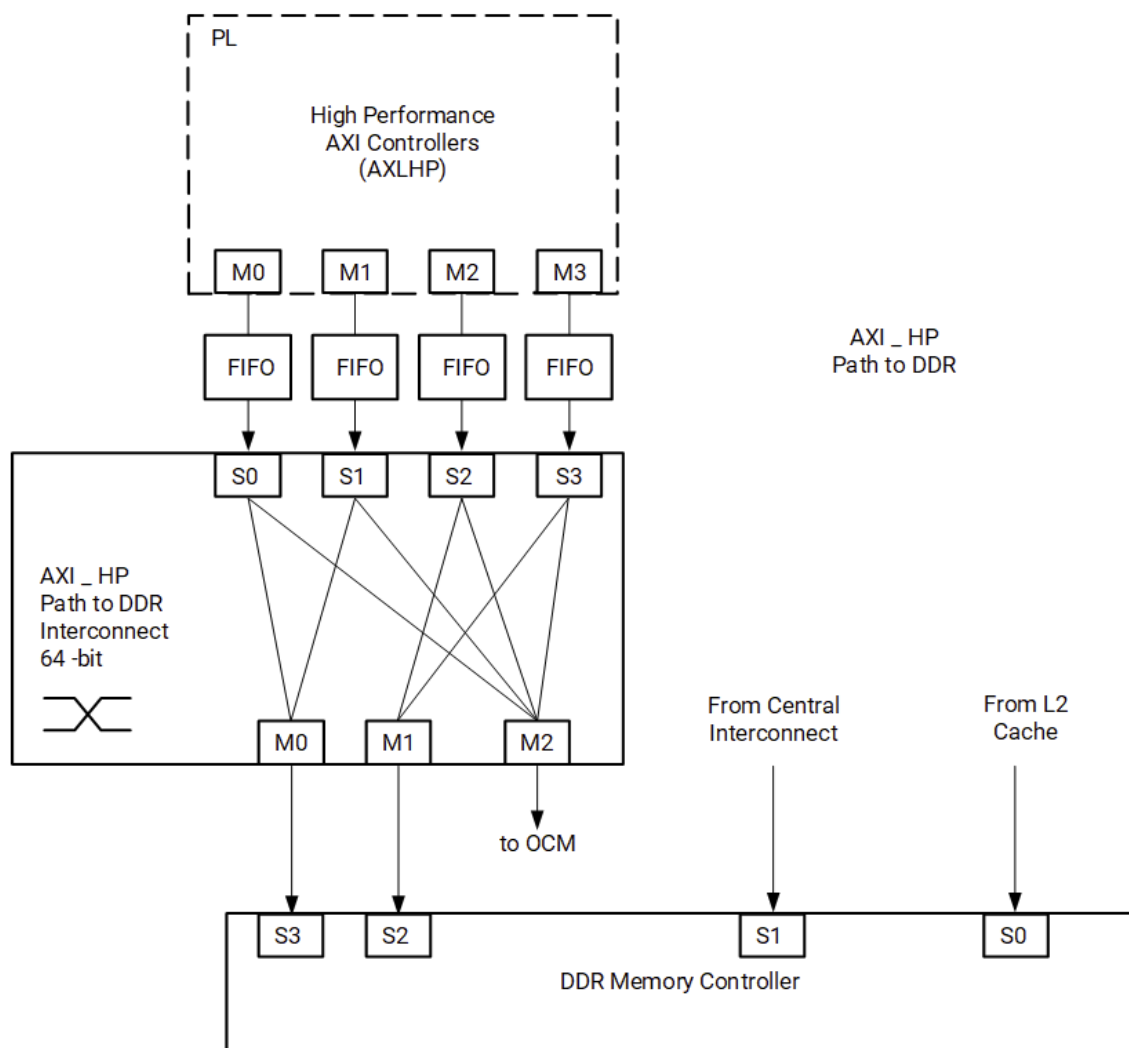
Figure: DDRC System Viewpoint
