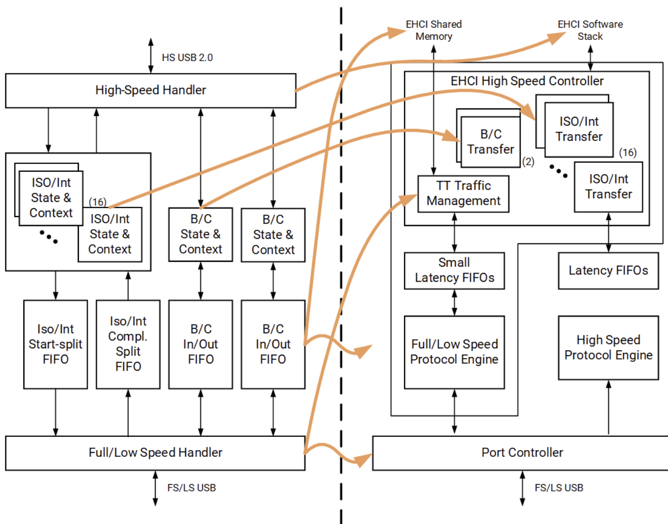
Figure: USB Host Embedded Transaction Translator Implementation
