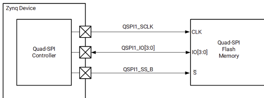
Figure: Quad-SPI Single SS 4-bit I/O
