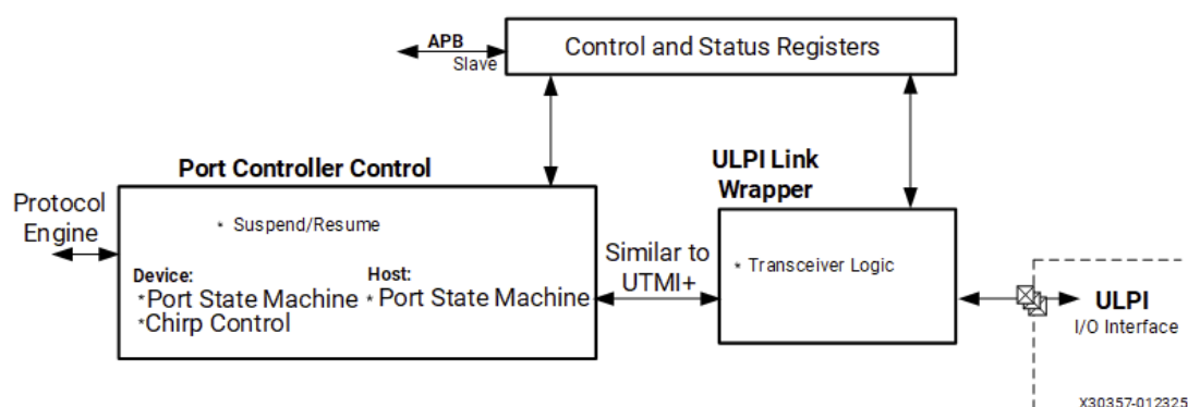
Figure: USB Port Controller and ULPI Link Wrapper Block Diagram
