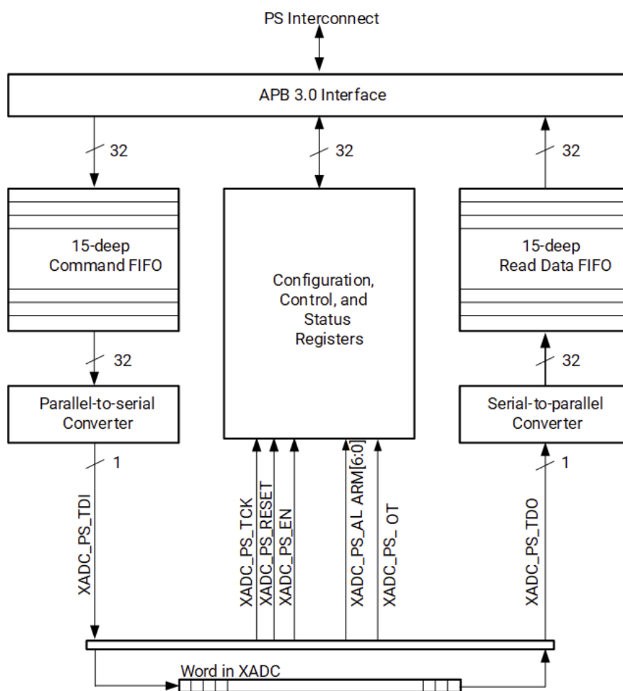
Figure: XADC PS-XADC Interface Block Diagram
