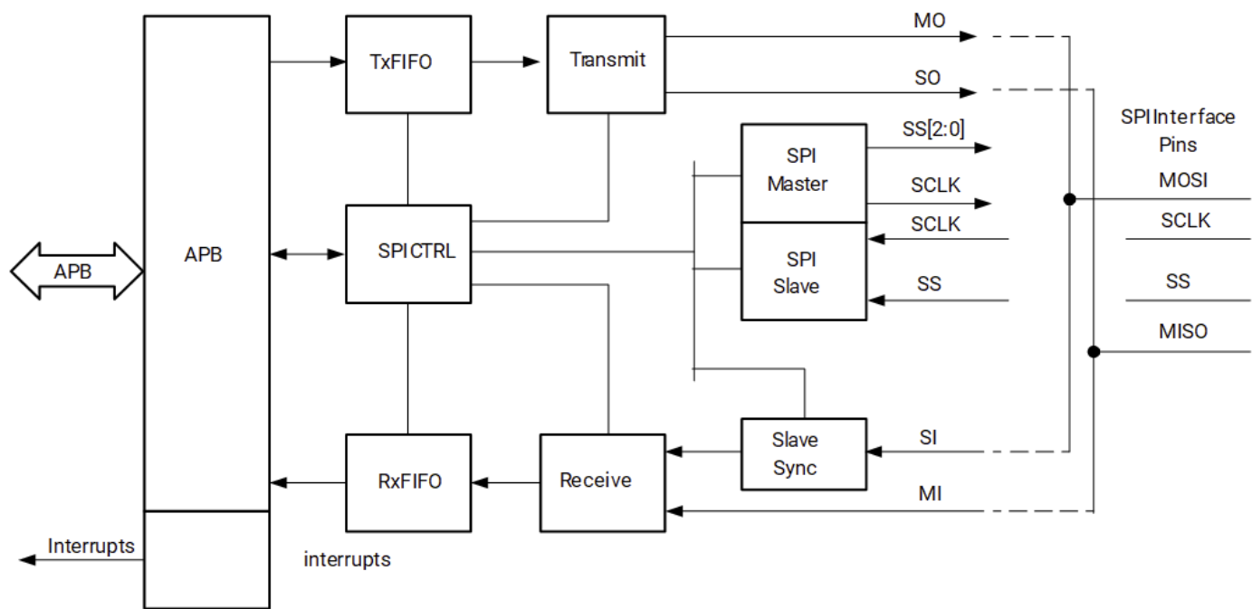
Figure: SPI Peripheral Block Diagram
