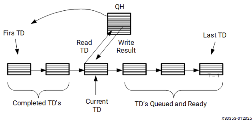
Figure: USB Controller Link-list Concept
