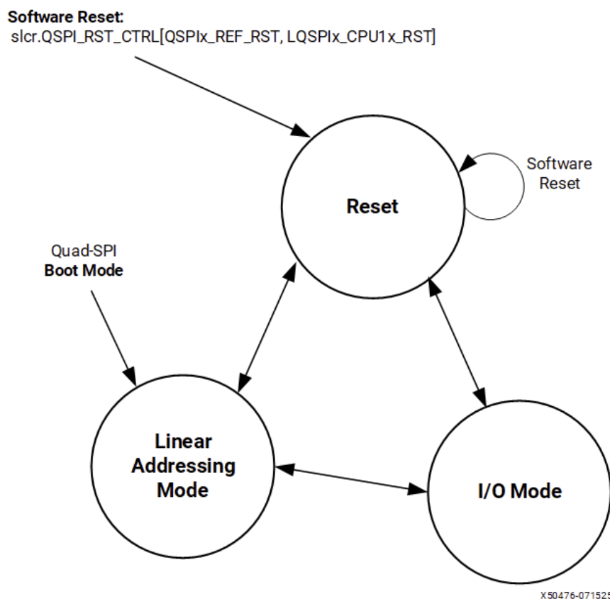
Figure: Quad-SPI Operating Mode Transitions
