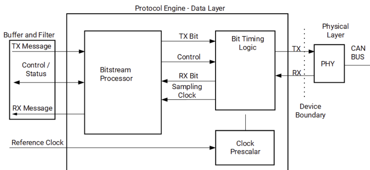
Figure: CAN Protocol Engine
