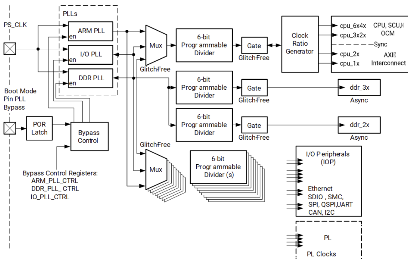
Figure: PS Clock System Block Diagram
