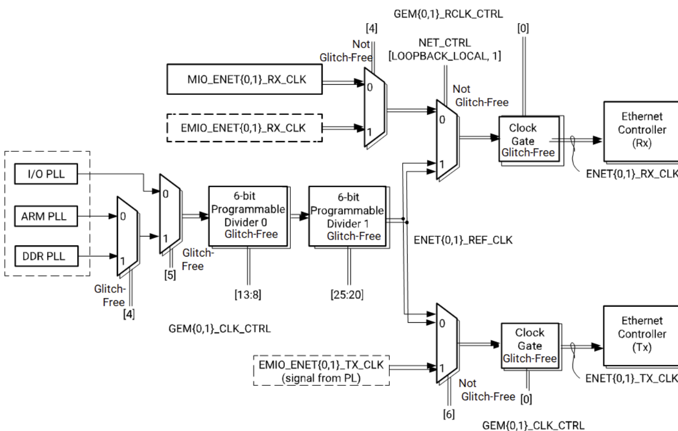
Figure: Ethernet Clock Generation
