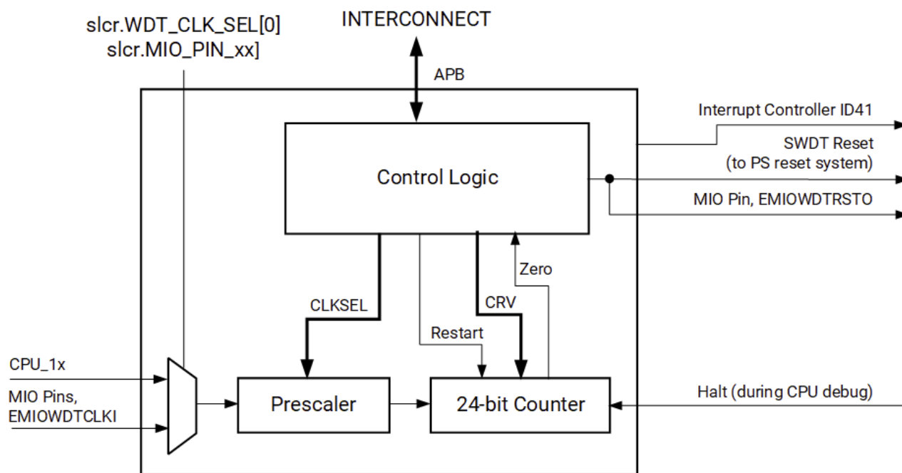
Figure: System Watchdog Timer Block Diagram
