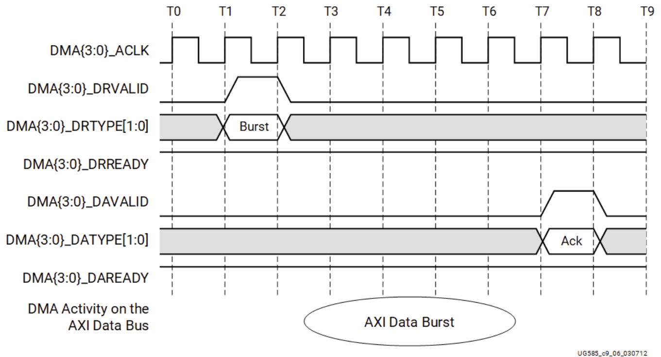
Figure: DMAC PL Peripheral Request Interface Burst Request Signaling
