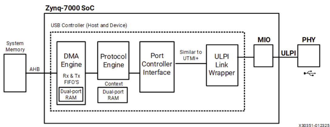
Figure: USB Controller Block Diagram
