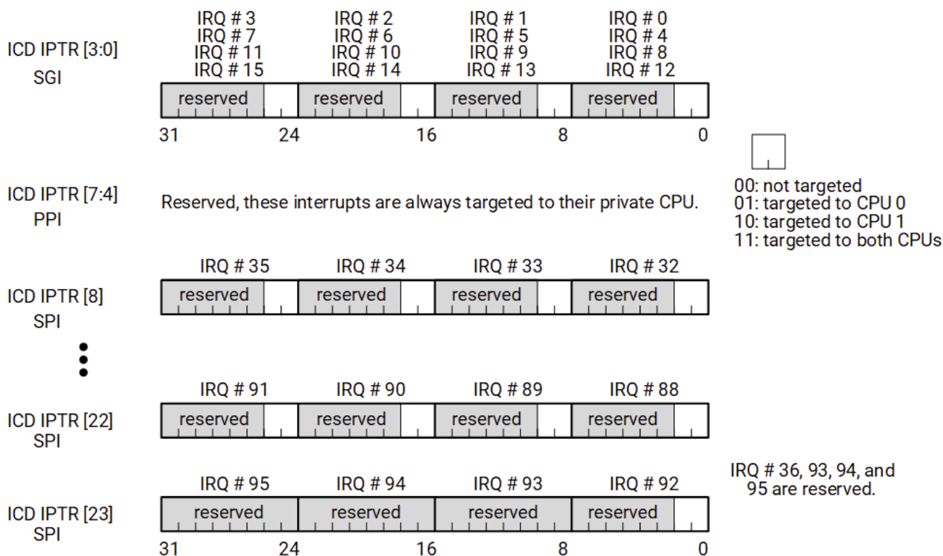
Figure: Interrupts ICDIPTR Register for Targeting CPU
