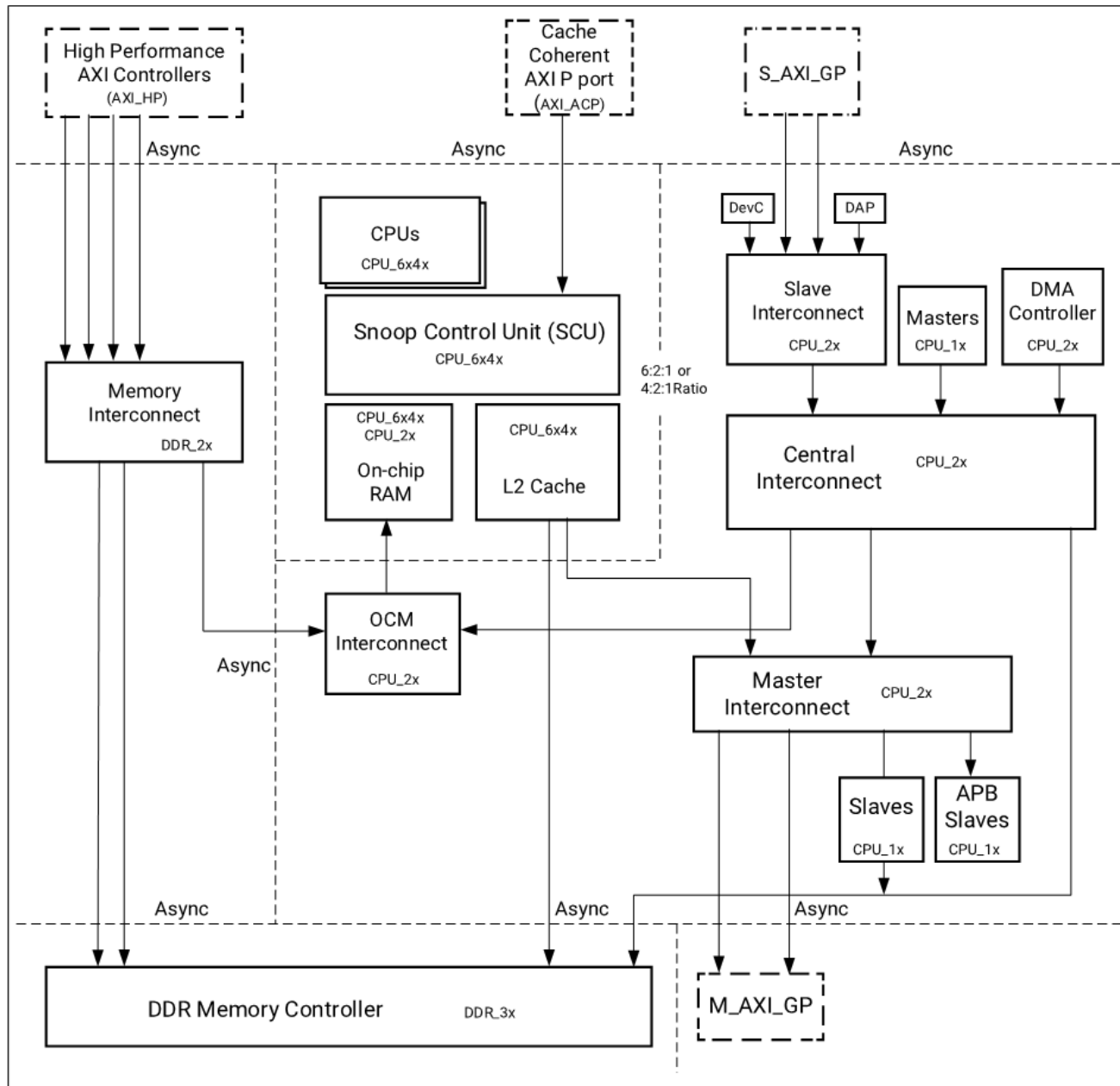
Figure: Interconnect Clock Domains
