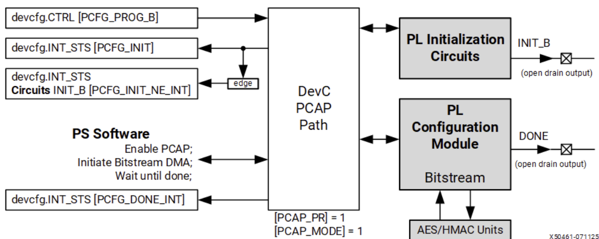
Figure: PCAP Path for PL Initialization and Configuration
