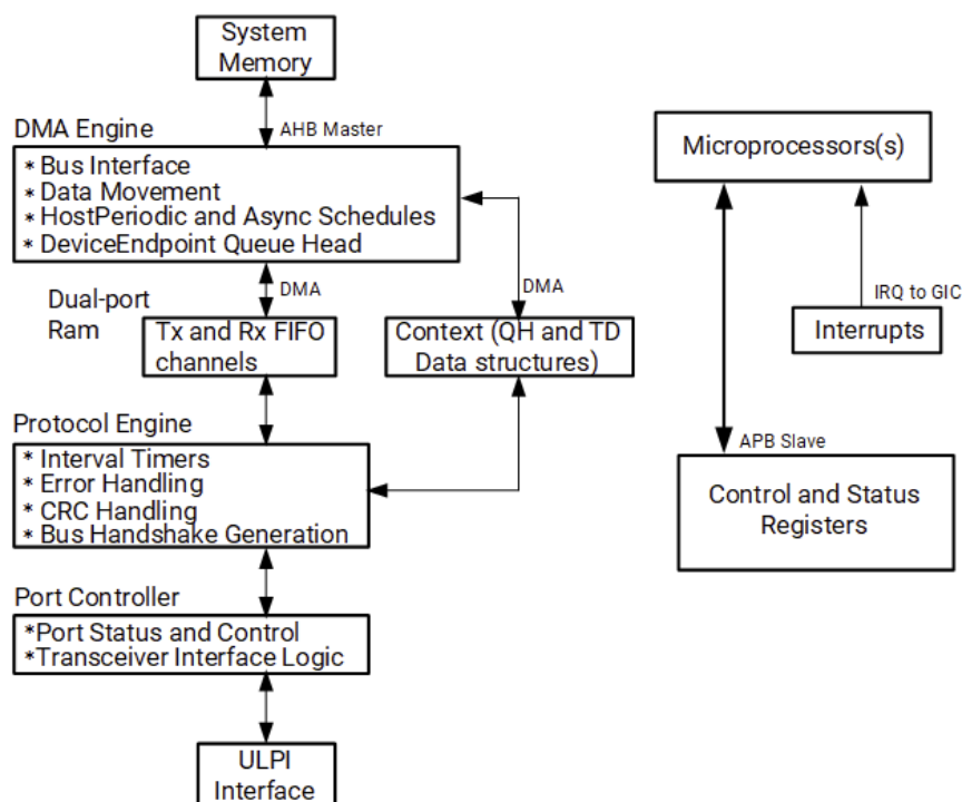
Figure: USB Controller Flow Diagram
