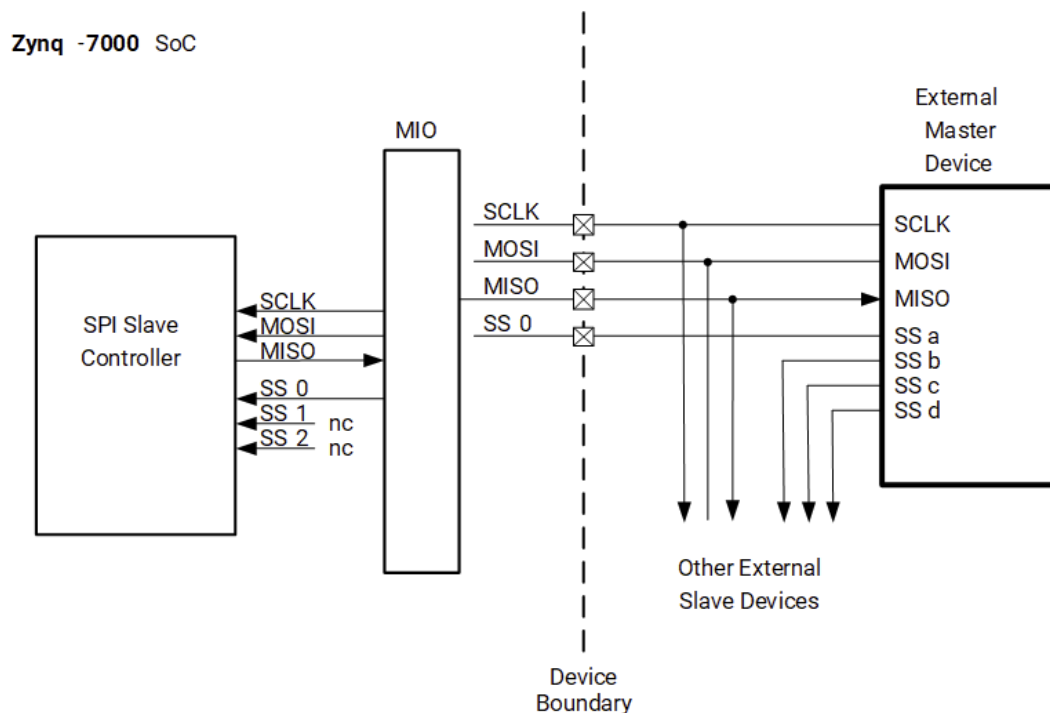
Figure: SPI Slave Mode Wiring Diagram via MIO
