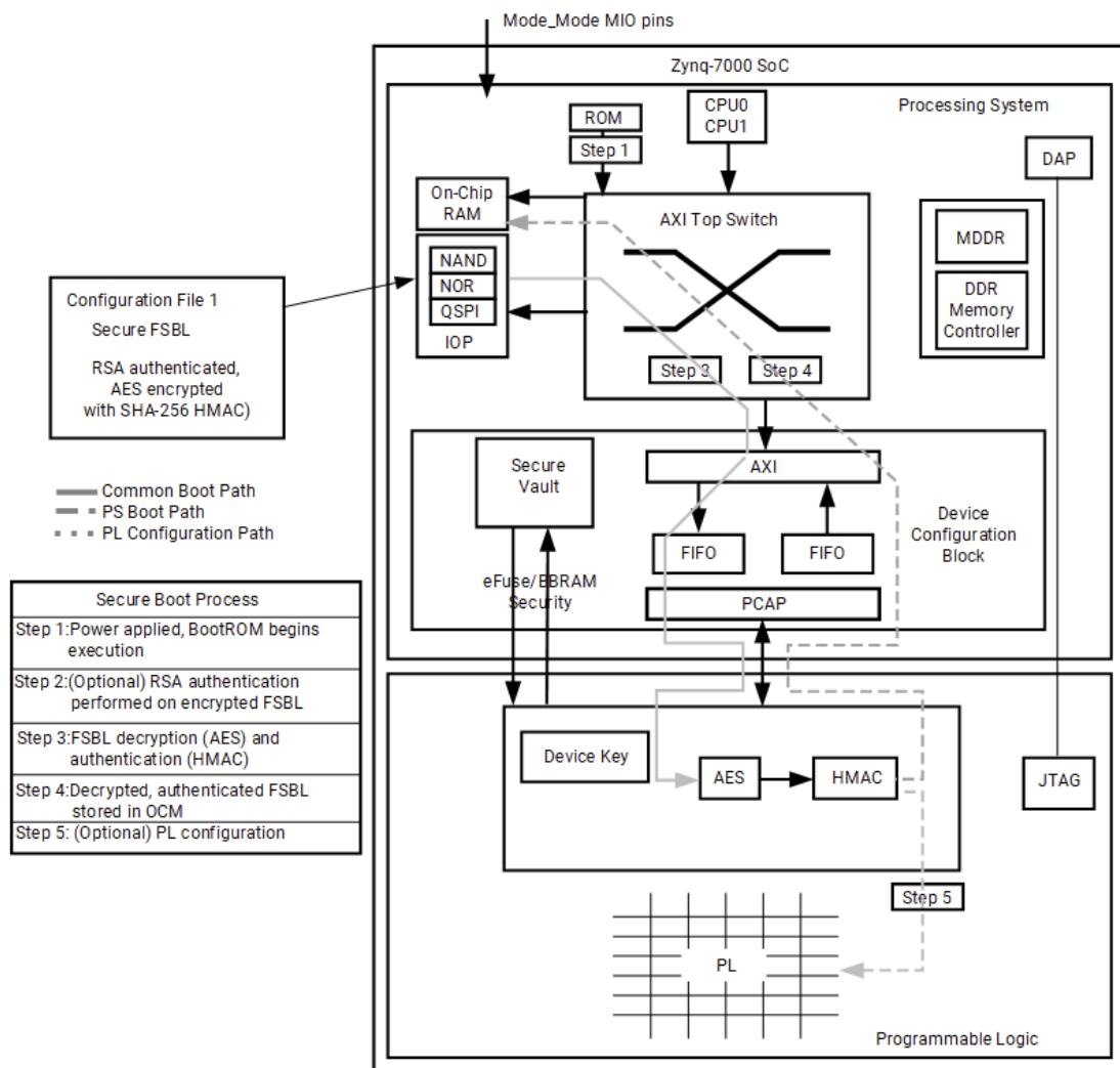
Figure: Secure Boot Block Diagram
