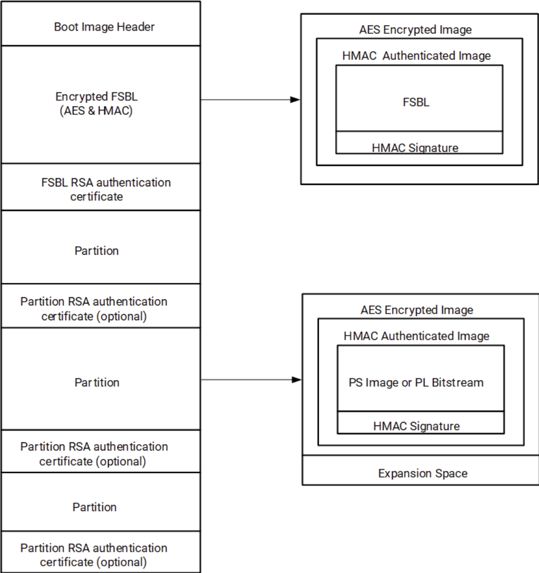
Figure: Secure Boot Image Format
