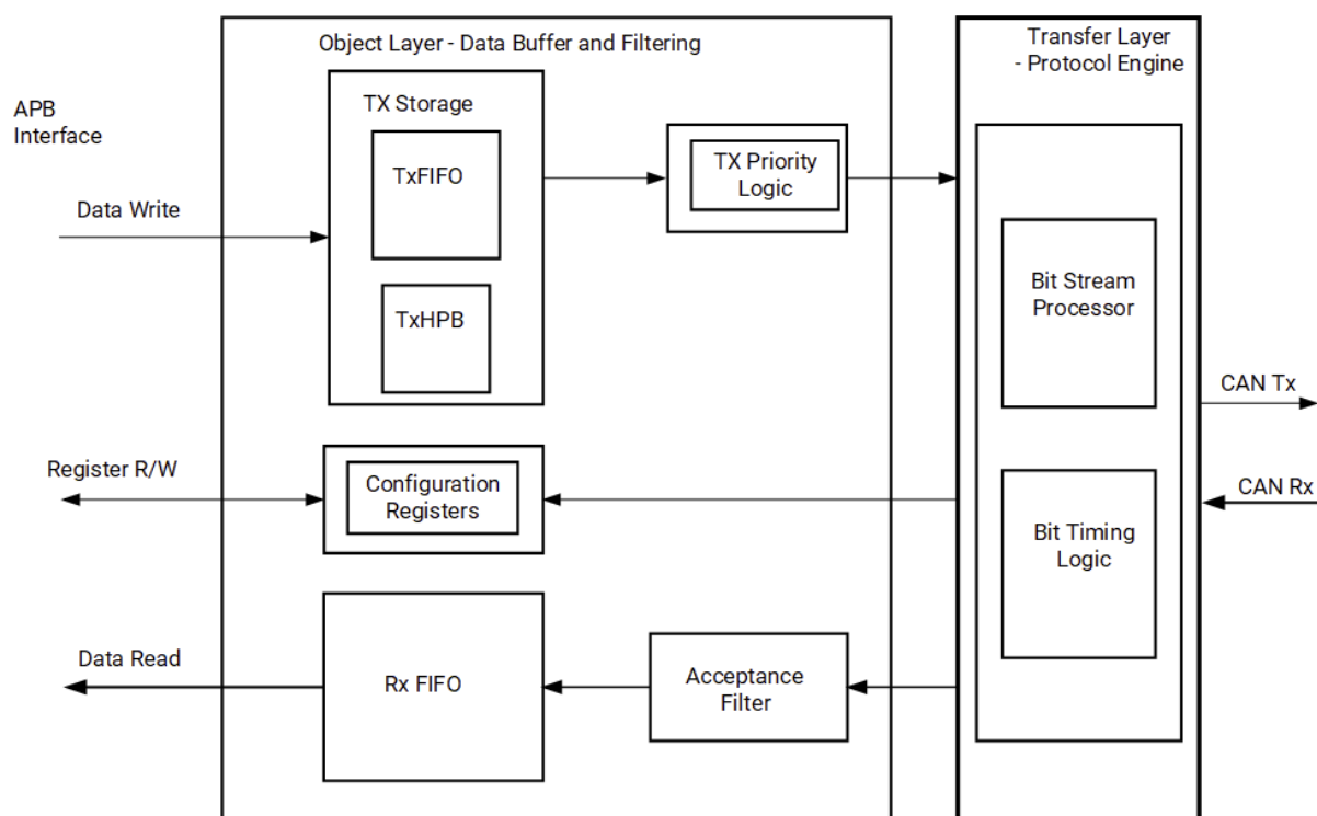
Figure: CAN Controller Block Diagram
