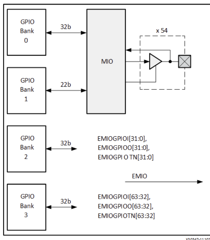
Figure: GPIO Block Diagram
