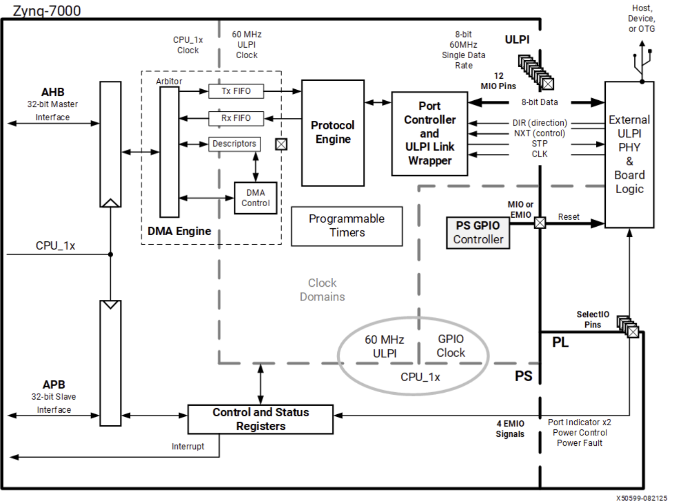
Figure: USB Detailed System Block Diagram
