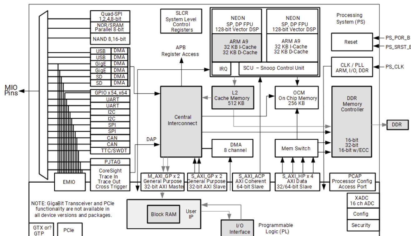
Figure: Example Cortex-A9 PL Data Movement Topology
