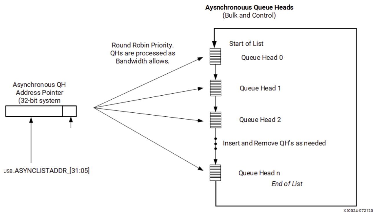
Figure: USB Host Controller Asynchronous Schedule Organization
