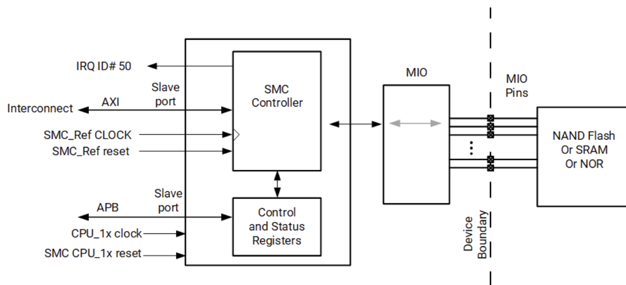
Figure: SMC System Level Diagram
