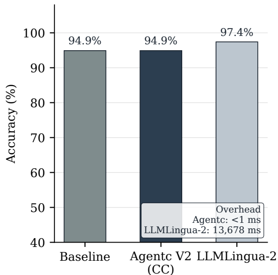
Natural prose (Wikipedia QA, n = 39 )
