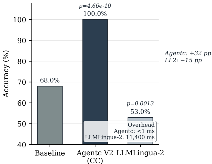
Distractor fixture (HotpotQA, n = 100 )
