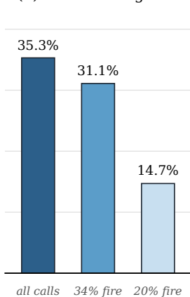
(b) ModelDowngrade
