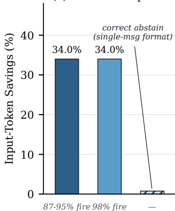
(a) ContextCompress
