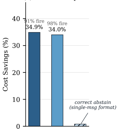
(a) ContextCompress
