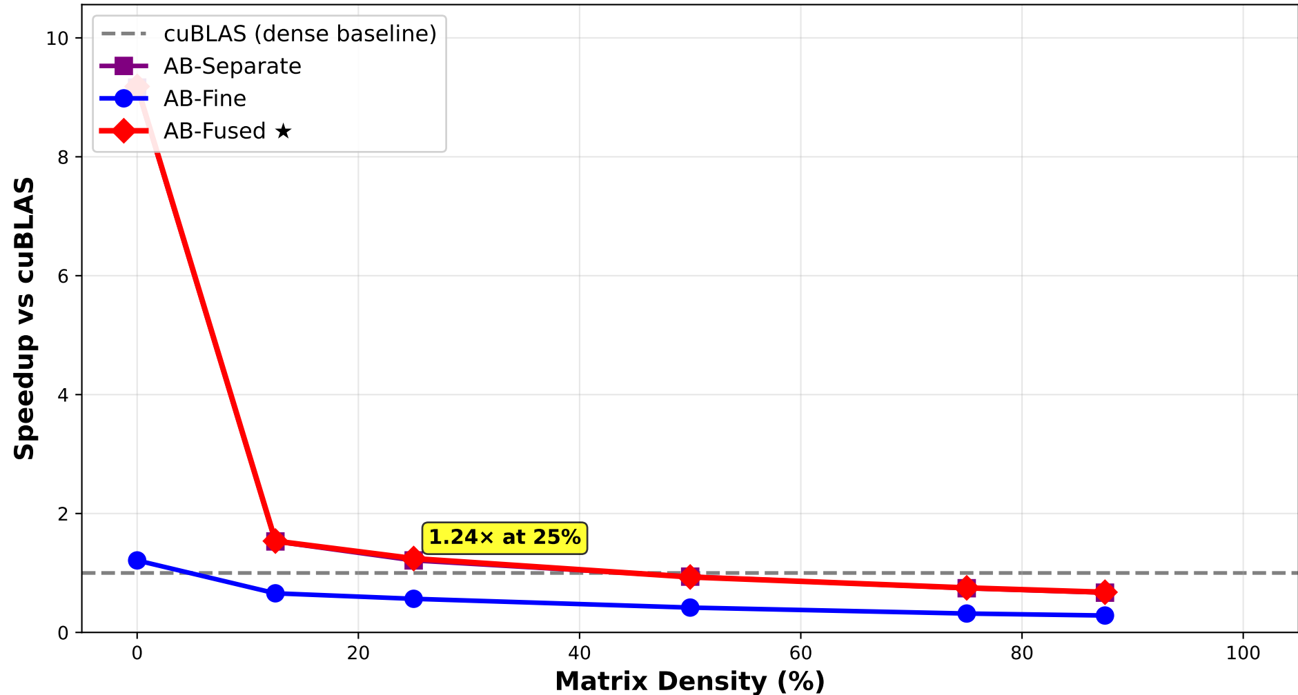
Figure 1: Performance vs Sparsity (4096×4096, blockwise sparsity)
