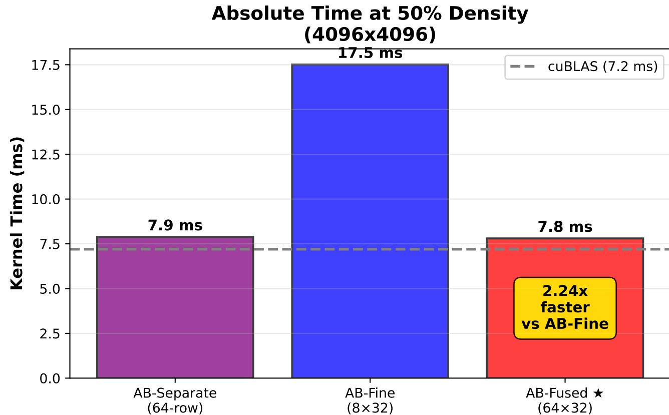
Figure 3: Fusion > Granularity (AB-Separate / AB-Fine / AB-Fused, 4096×4096)
