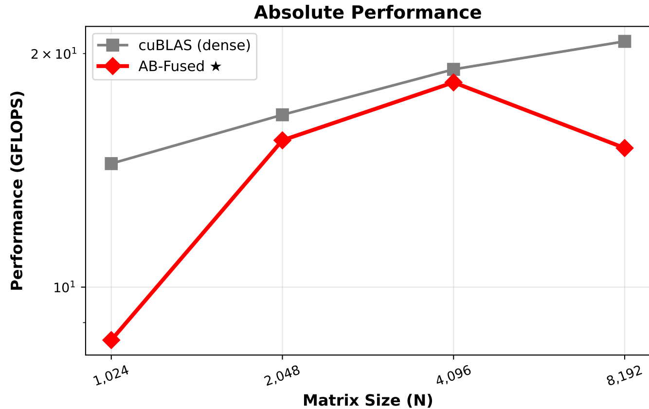
Figure 5: Matrix Size Scaling (AB-Fused vs cuBLAS, 50% density)
