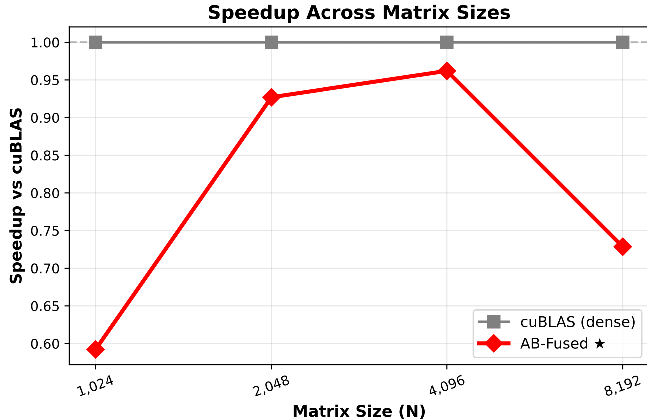
Figure 5: Matrix Size Scaling (AB-Fused vs cuBLAS, 50% density)
