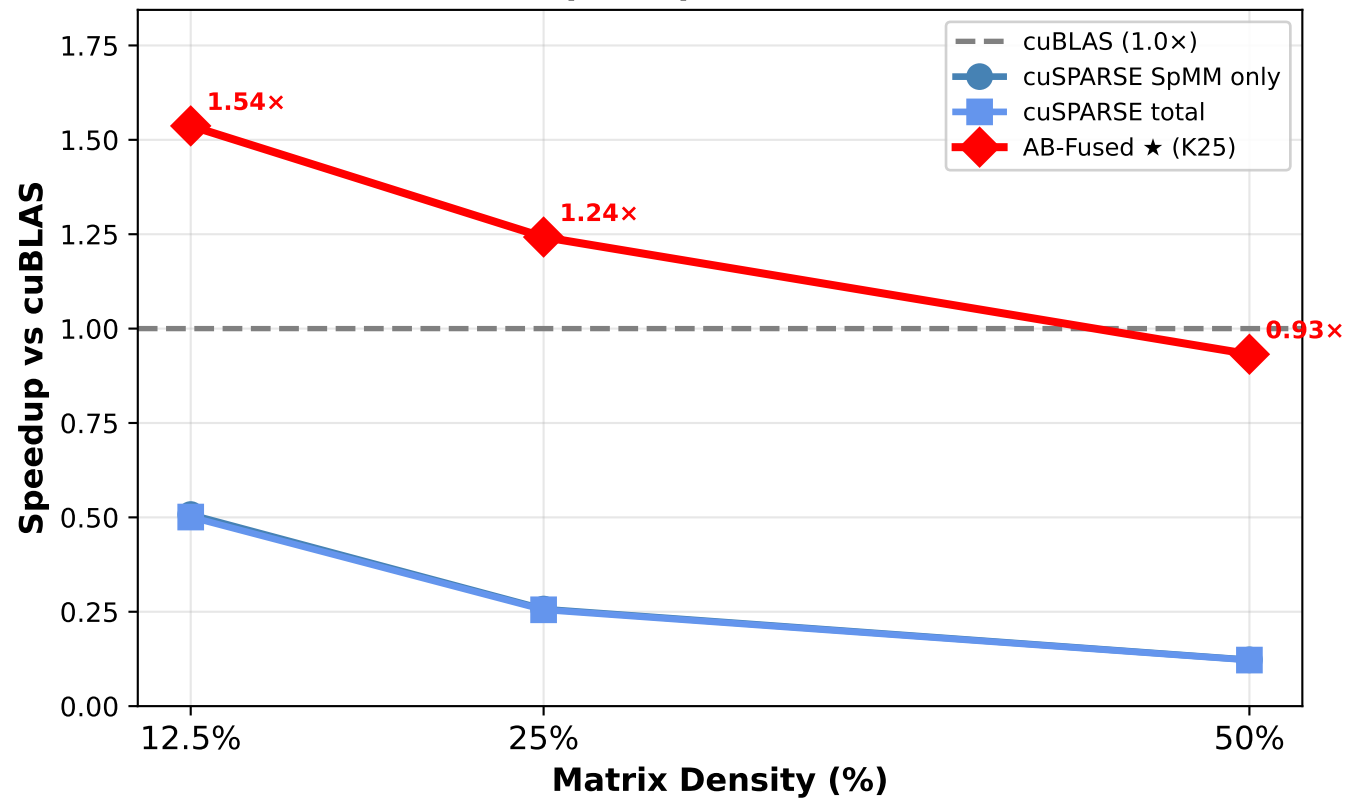
Speedup vs cuBLAS
