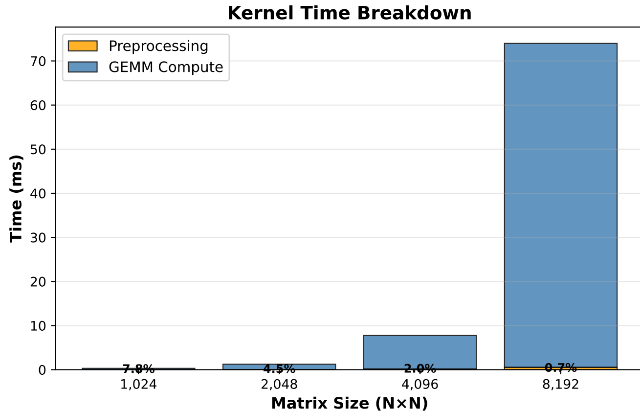
Figure 2: K25 Preprocessing Overhead (50% density)
