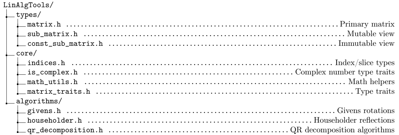
Figure 2: Directory structure of the LinAlgTools library
