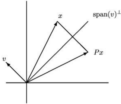
Figure 1: Householder reflection applied to vector x
