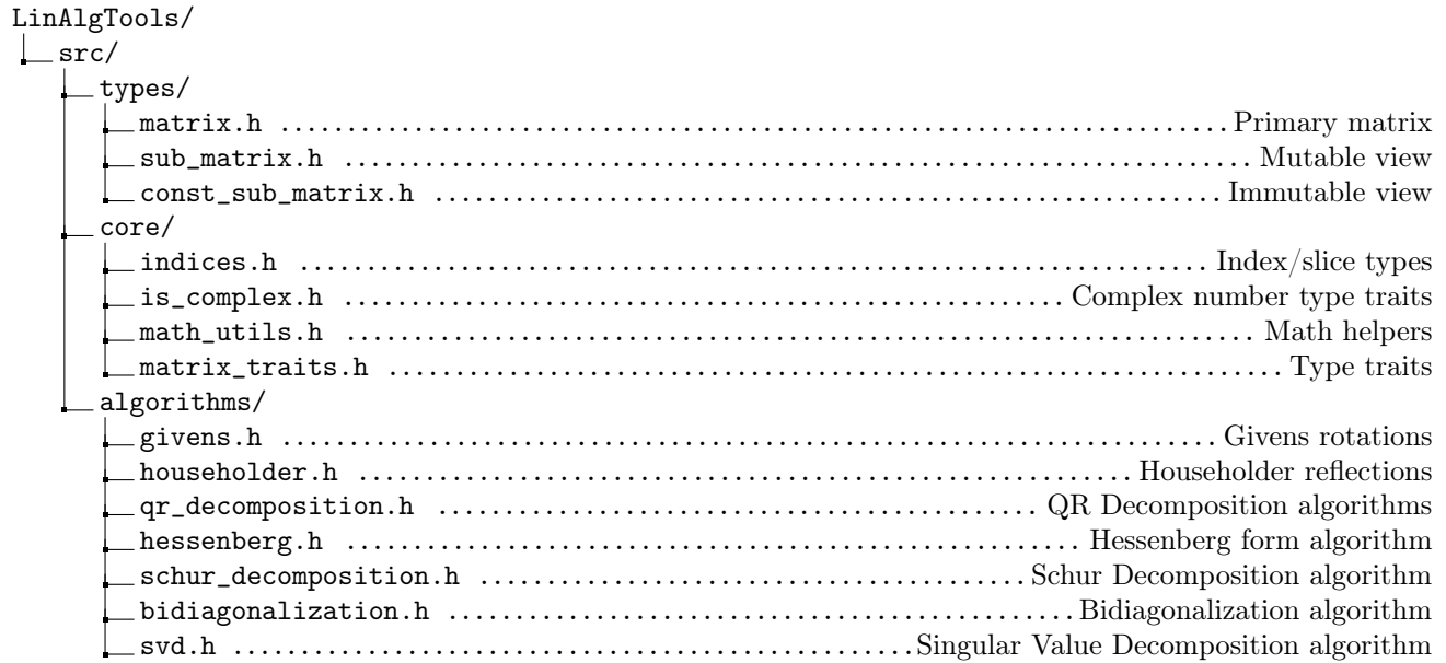
Figure 2: Directory structure of the LinAlgTools library
