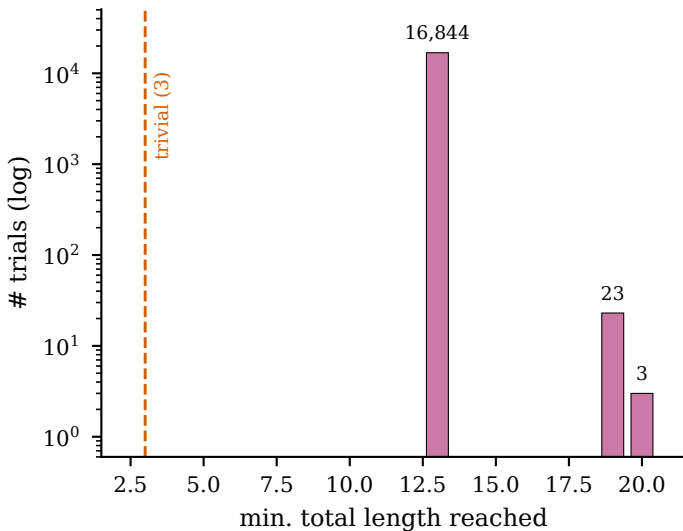
Lane-D campaign: 16,870 trials, 0 solved
