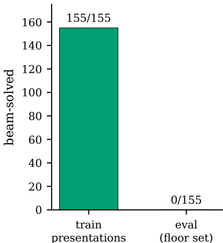
RL train vs. floor eval
