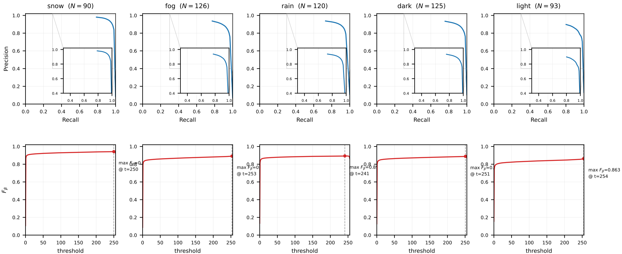
Reported model — threshold behaviour on real-world test ( F_\beta , \beta^2 = 0.3 )
