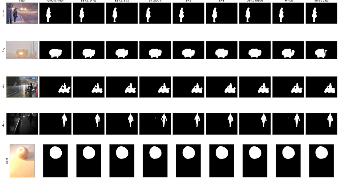
Figure 4. The same scenes predicted by eight different trained arms. Rows are the five real-world test conditions, easiest to hardest by MAE: snow, fog, rain, dark and light. The first two columns are the input and the ground truth; the remaining eight are arms drawn from Table 4 spanning the widest architectural spread the study contains — the reported model, the ablation reference, a 14-epoch run, an E=2 model, an E=4 k=1 model, a single-dense-expert model, the no-mixture model, and the dense-gate model. Every one of those eight columns is a different model; the masks are nonetheless indistinguishable, and the two columns that do differ from the rest are the input and the ground truth. This is the ablation result of Table 4 rendered as an image, and it is the reason the paper reports a null result rather than a design win.
