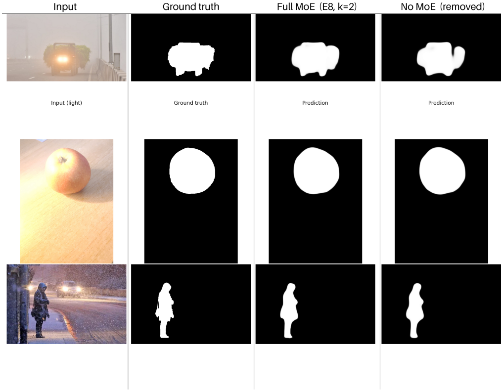
Figure 5. The mixture-of-experts does not change the prediction. Read the four columns left to right: (1) input , (2) ground truth , (3) full MoE (E8, k=2 , 14 epochs) and (4) no MoE (the identical architecture with the mixture removed). Columns 3 and 4 are therefore two different models on the same image; both are labelled “Prediction” inside the grid because that is how the evaluation tool renders a single model’s output. Rows are real-world test images under fog, light and snow. The two prediction columns are indistinguishable in the light row; in the fog and snow rows the differences are confined to object boundaries. This is the qualitative counterpart of the no-MoE row in Table 4, where removing the MoE leaves real-test MAE unchanged at 0.0195.
