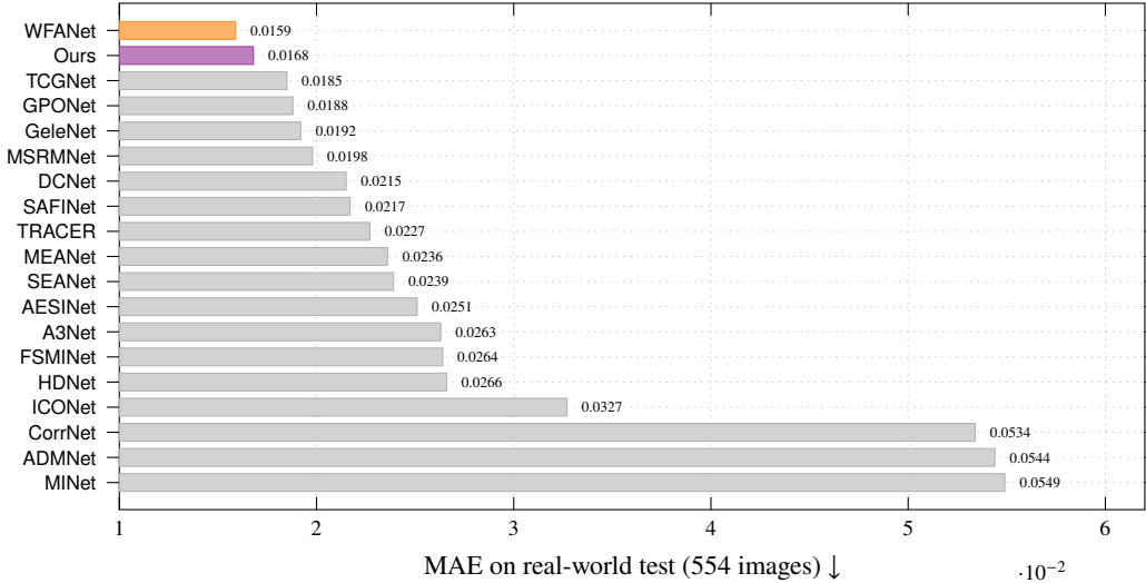
Figure 3. Real-split accuracy ranking. All nineteen entries of the WXSOD benchmark tables, ordered by MAE. Grey: the 17 published SOD methods; orange: WFANet, the benchmark’s weather-supervised baseline; violet: ours. Every published value is as reported in [7] under the authors’ own protocol; only the violet bar is measured in this work. Our model uses no weather labels at training or inference, whereas WFANet uses nine-class weather supervision. The horizontal axis starts at 0.010 rather than 0 so that the ranking is legible; it is not a zero-based scale.
