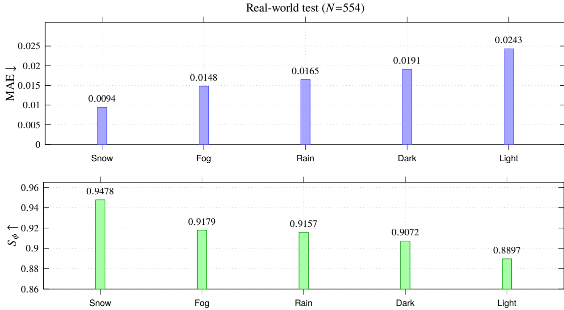
Figure 6. Weather-wise accuracy on real-world test. Top: MAE; bottom: S_\phi . Snow is the easiest condition and light the hardest, a 2.6\times spread in MAE. Condition names are the dataset’s own labels and are reported verbatim.
