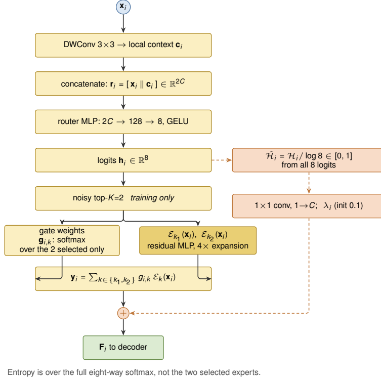
Figure 2. Routing for one token at one pyramid scale. A depthwise 3 \times 3 convolution supplies local context, which is concatenated with the token and passed through a two-layer MLP to give eight routing logits. Input-dependent Gaussian noise is added during training; top- K=2 then selects two experts, and the gate weights are a softmax over those two logits only. Each selected expert is a residual MLP with a 4 \times channel expansion. Routing entropy is taken over the full eight-way distribution, not the selected pair, and the normalised value is projected and added to the decoder feature.
