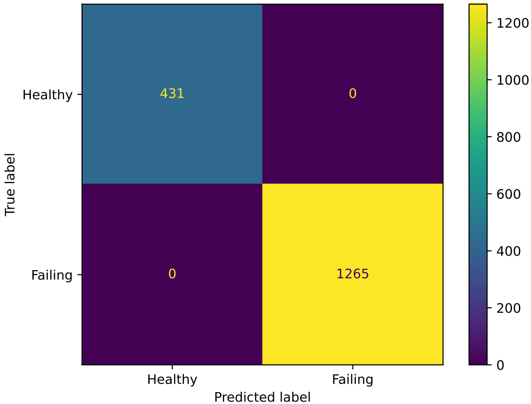
Confusion Matrix - Bearing Classification
