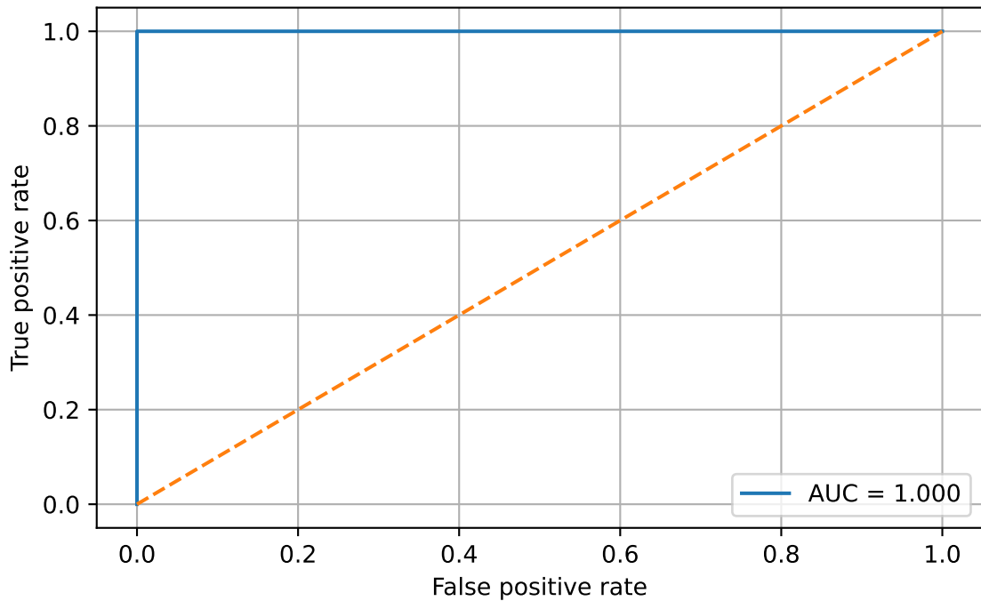
ROC Curve - Bearing Failure Detection
