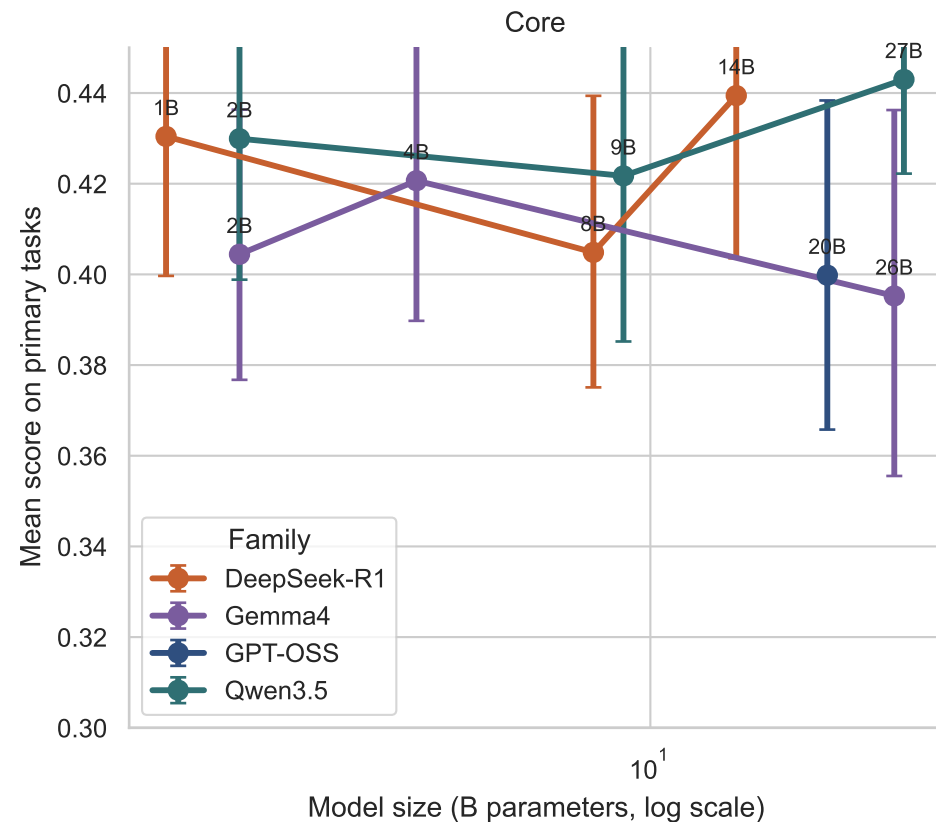
Frozen scaling profile on the primary latent-adaptation tasks (95% bootstrap CIs)
