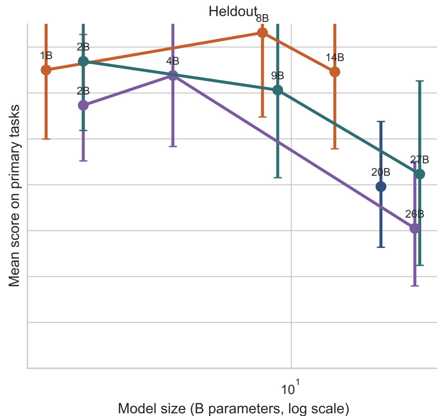
Frozen scaling profile on the primary latent-adaptation tasks (95% bootstrap CIs)
