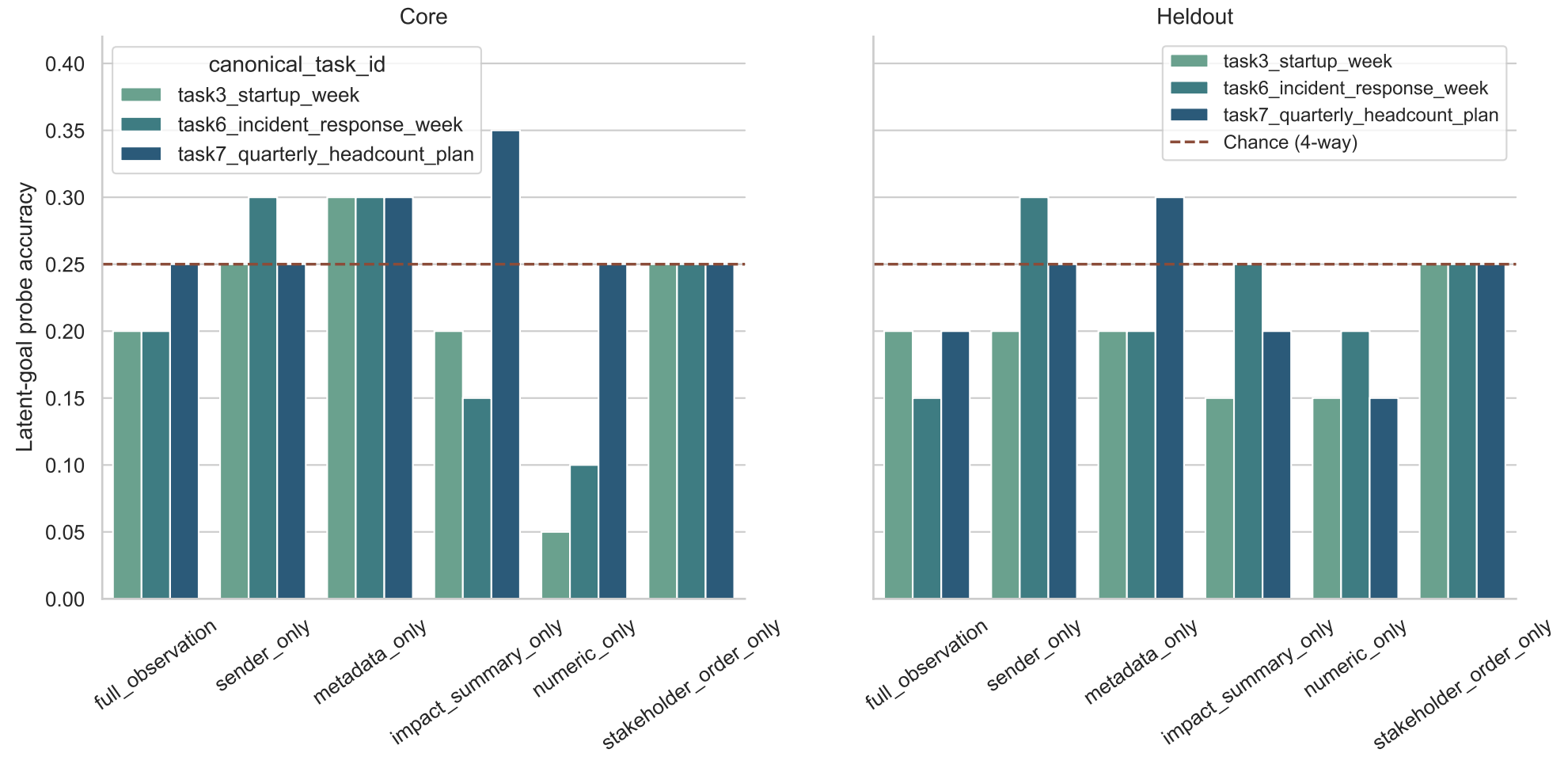
Restricted-view leakage probes stay near 4-way chance on the primary tasks
