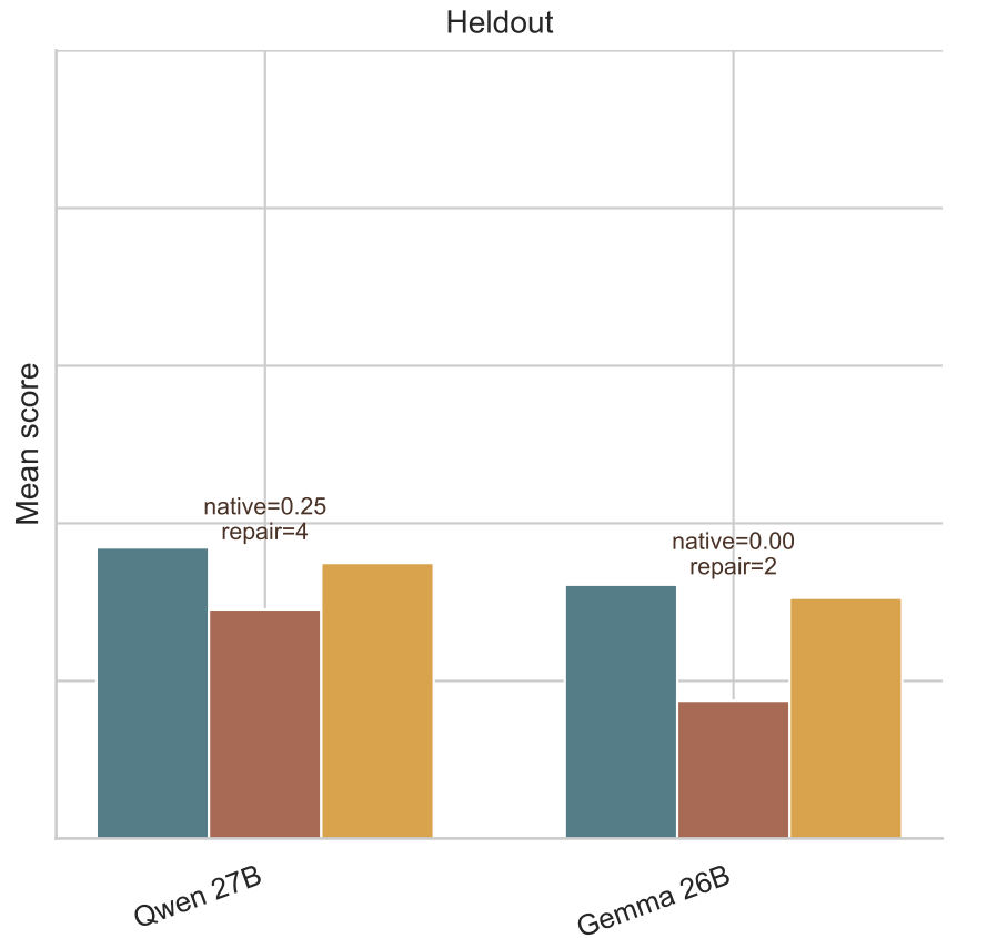
Shell-controlled appendix diagnostic: lightweight parse repair only partially rescues Qwen-27B and does not rescue Gemma-26B
