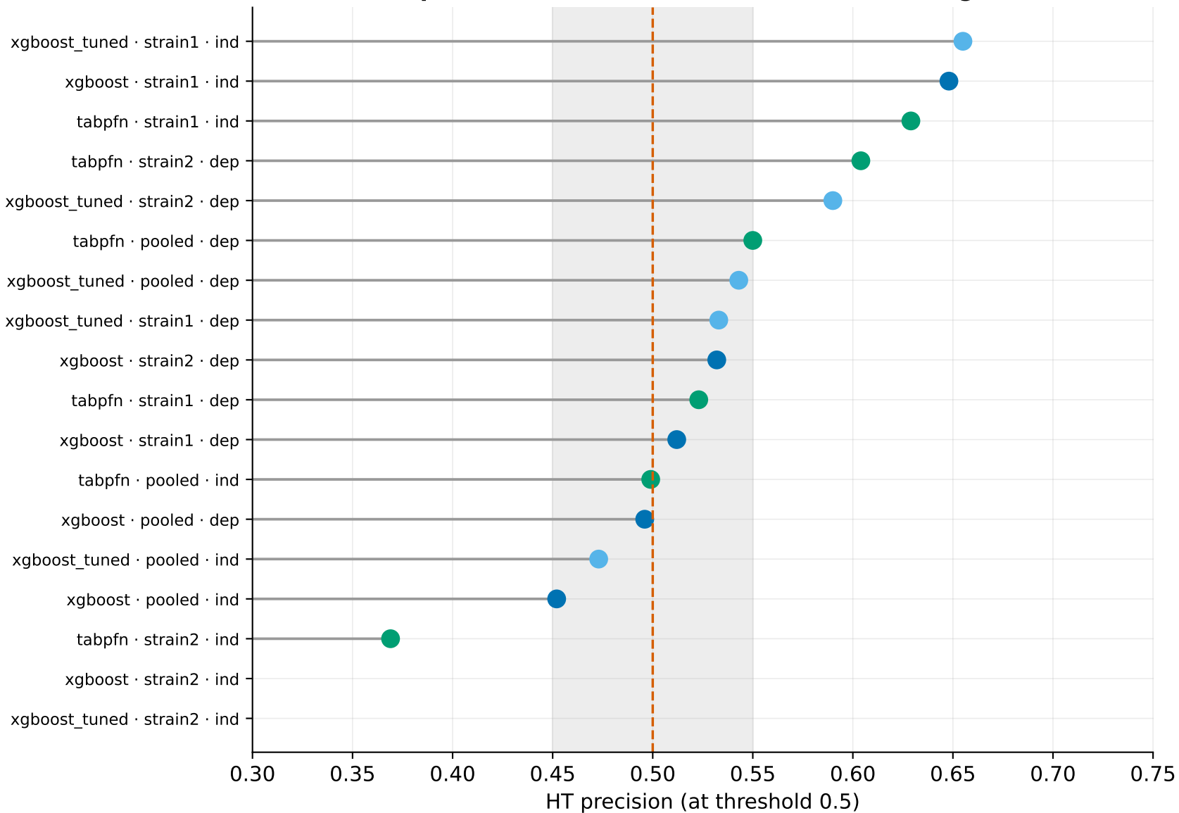
The HT-precision wall (~0.50) across tabular configurations
