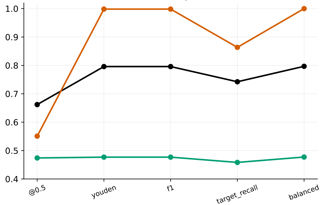
TabPFN · independent
