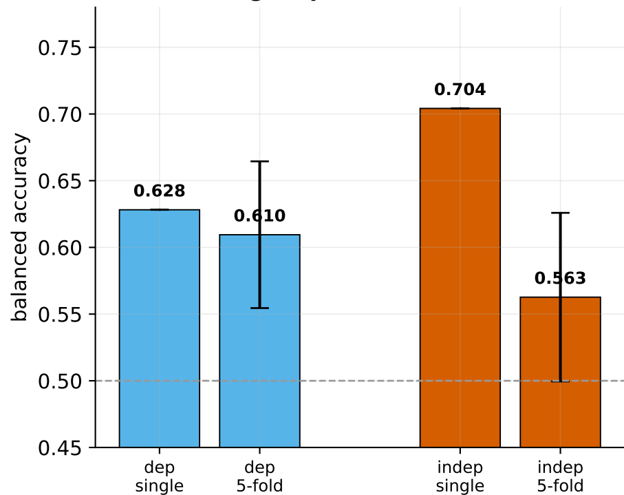
BiLSTM (balanced sampler): single-split vs 5-fold CV
