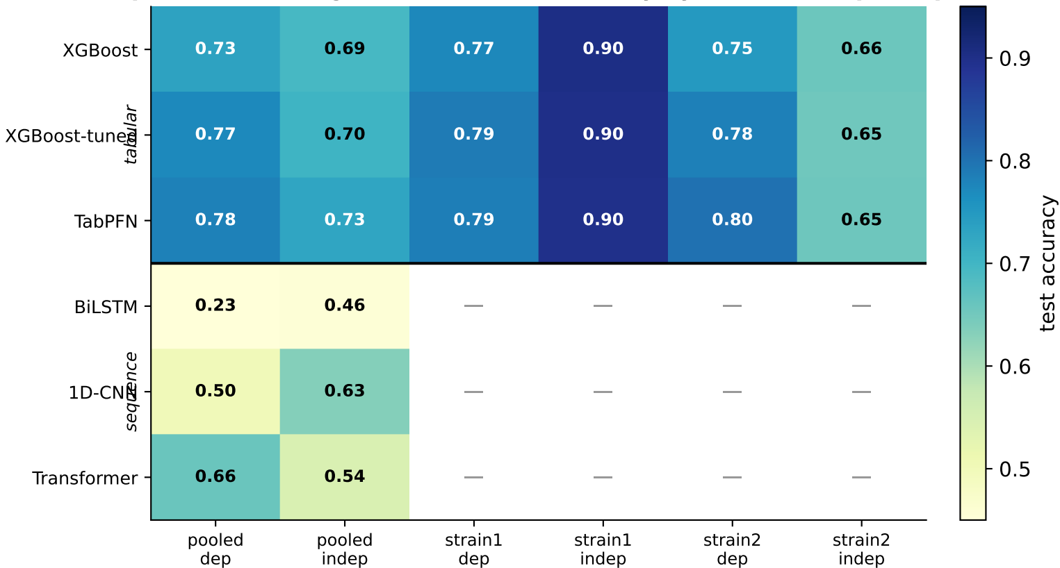
Experimental-design matrix — test accuracy by model × scope × split
