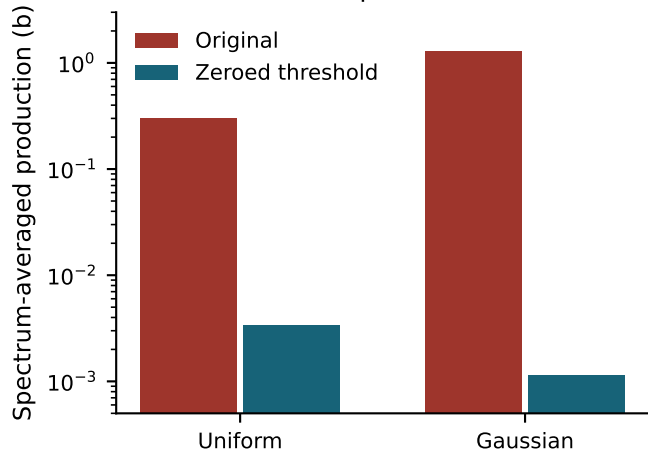
(b) Cl-35 spectrum folds
