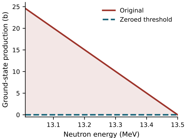
(a) Cl-35 first interval
