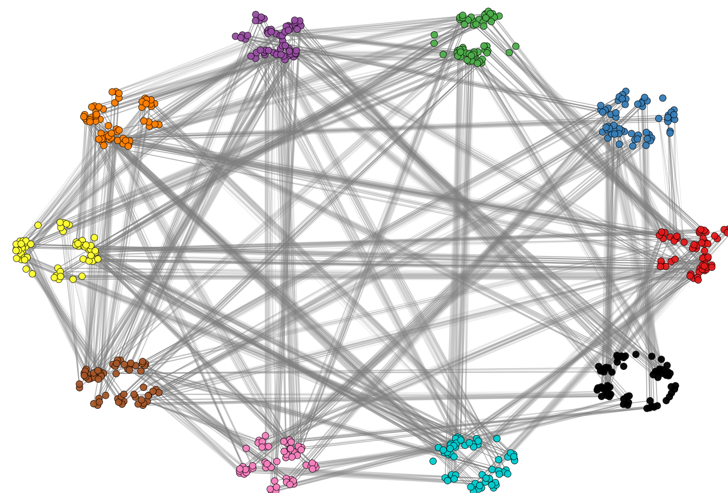
Combo LRC→ORC sparsification E=11661, reduction=40.1%
