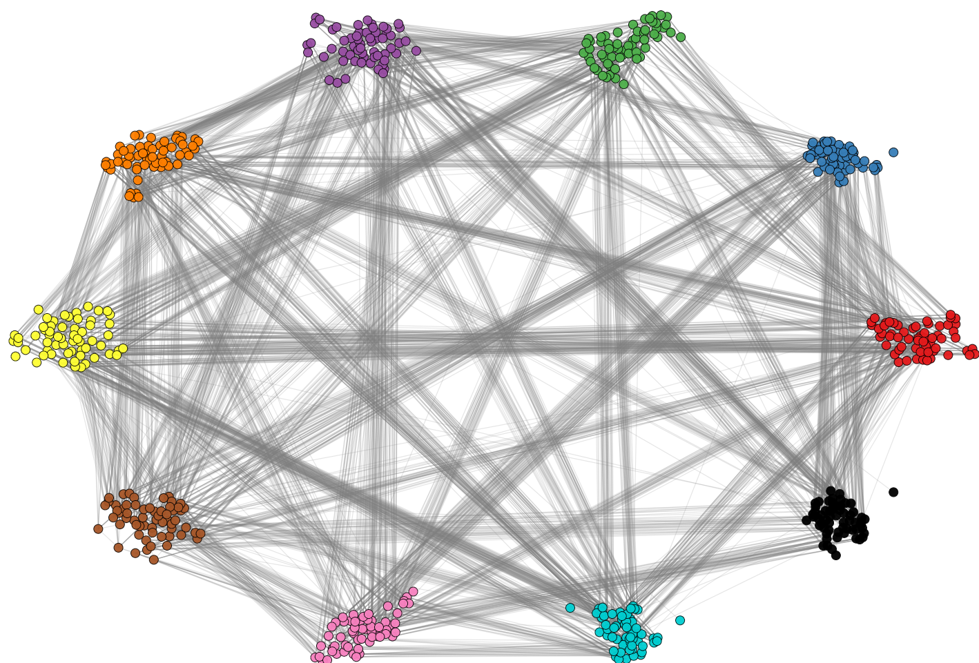
ORC-only sparsification E=14597, reduction=25.0%
