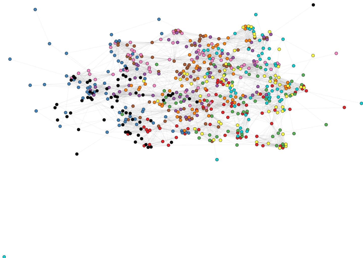
ORC-only sparsification E=14597, reduction=25.0%
