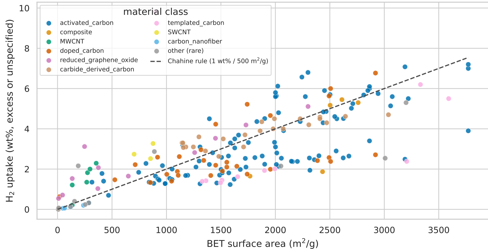
The Chahine rule across material classes (77 K)
