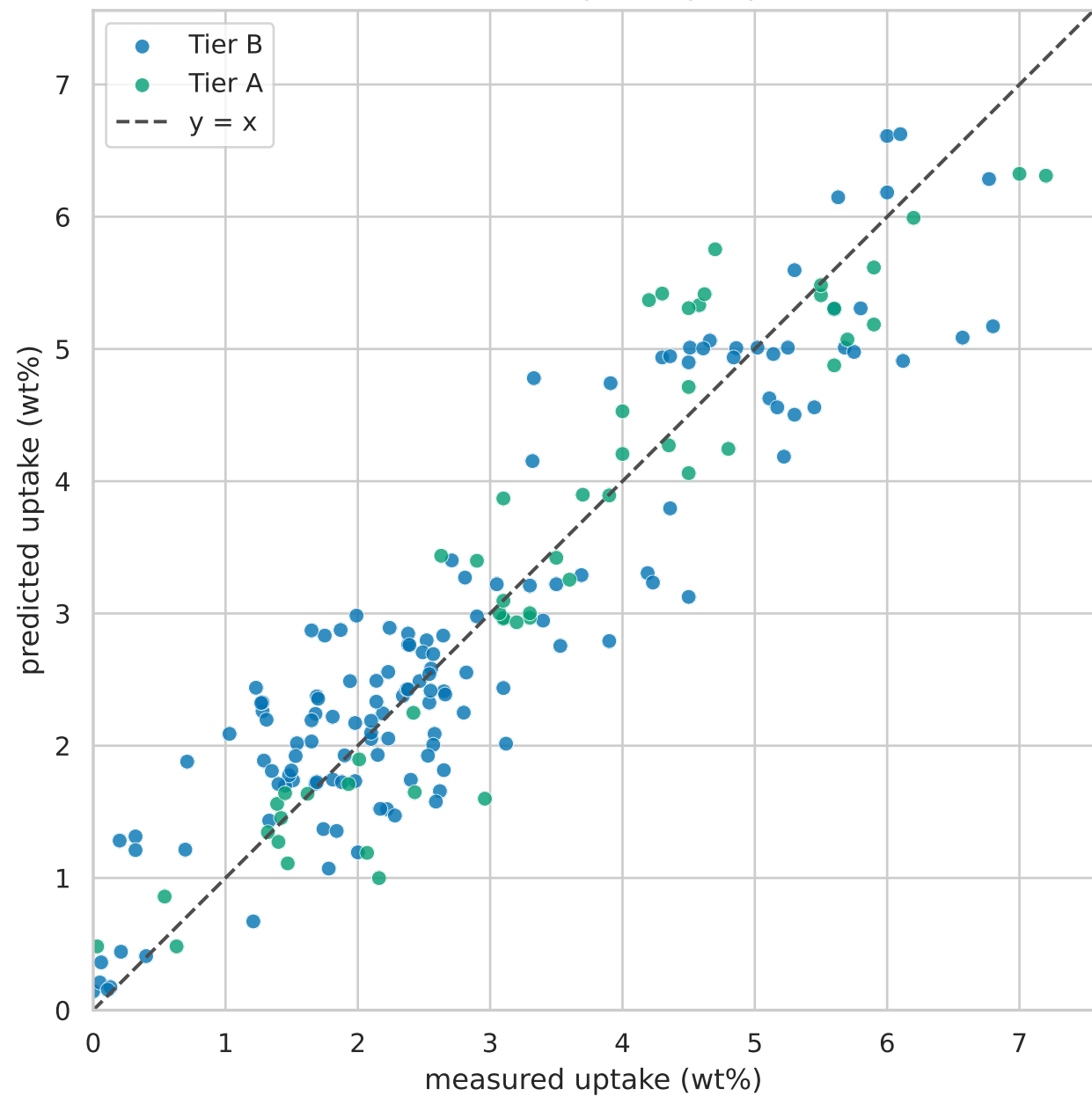
Predicted vs measured H 2 uptake (grouped CV, XGBoost)
