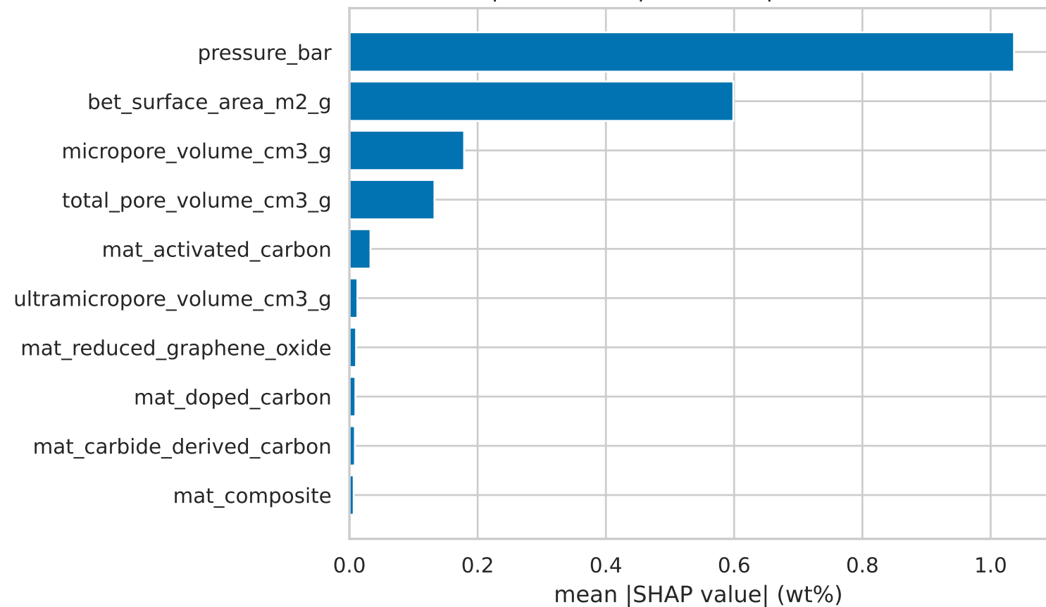
Feature importance for predicted uptake (SHAP, XGBoost)
