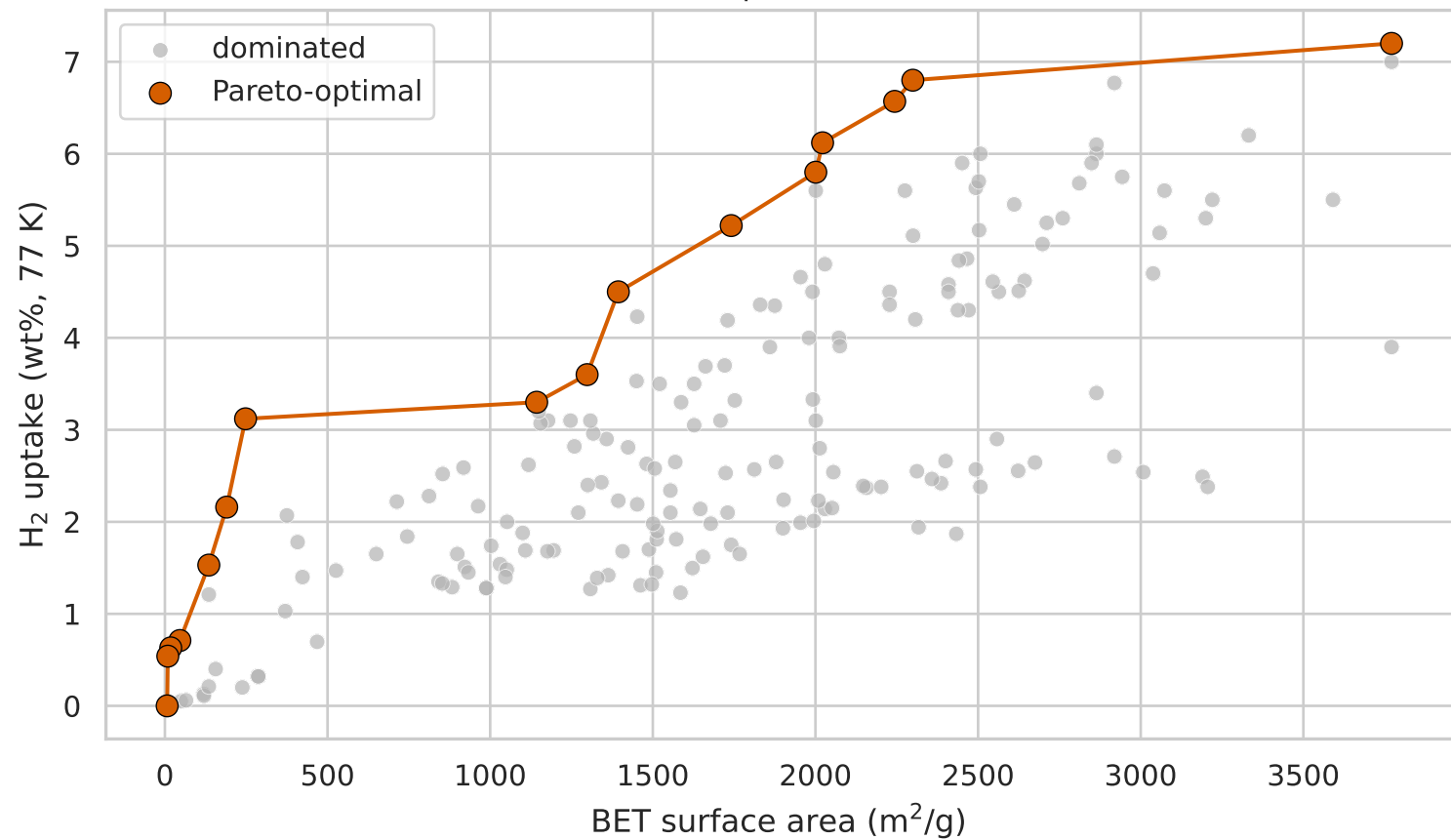
Materials trade-off: most uptake for the least surface area
