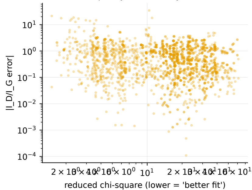
(a) Fit quality vs accuracy (SNR 50)
