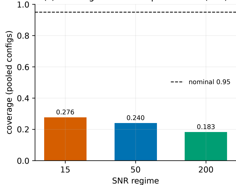
(c) Coverage under misspecification (T6b)
