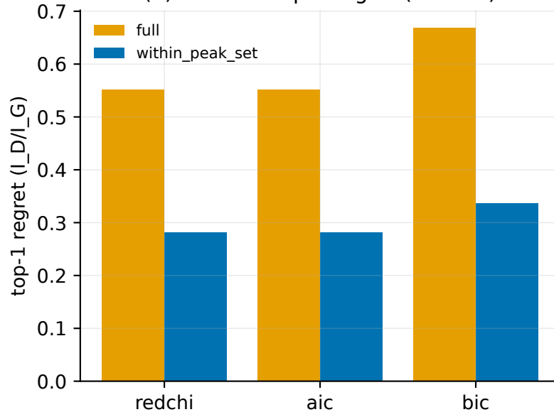
(b) Selector top-1 regret (SNR 50)
