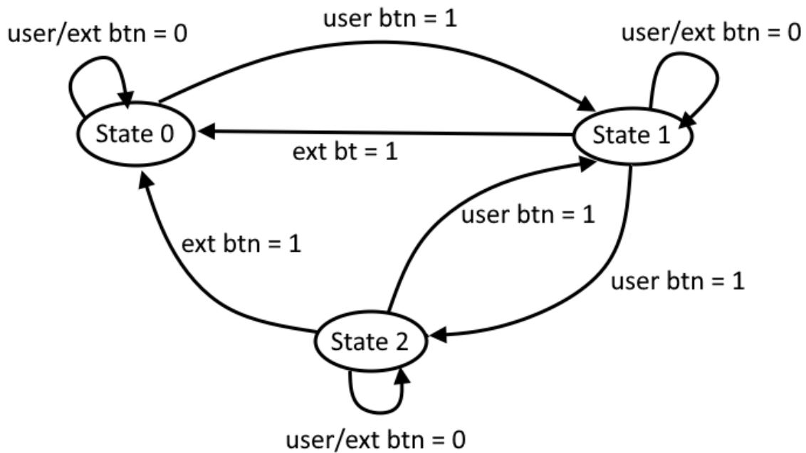
Figure 1: Diagram for Finite State Machine
