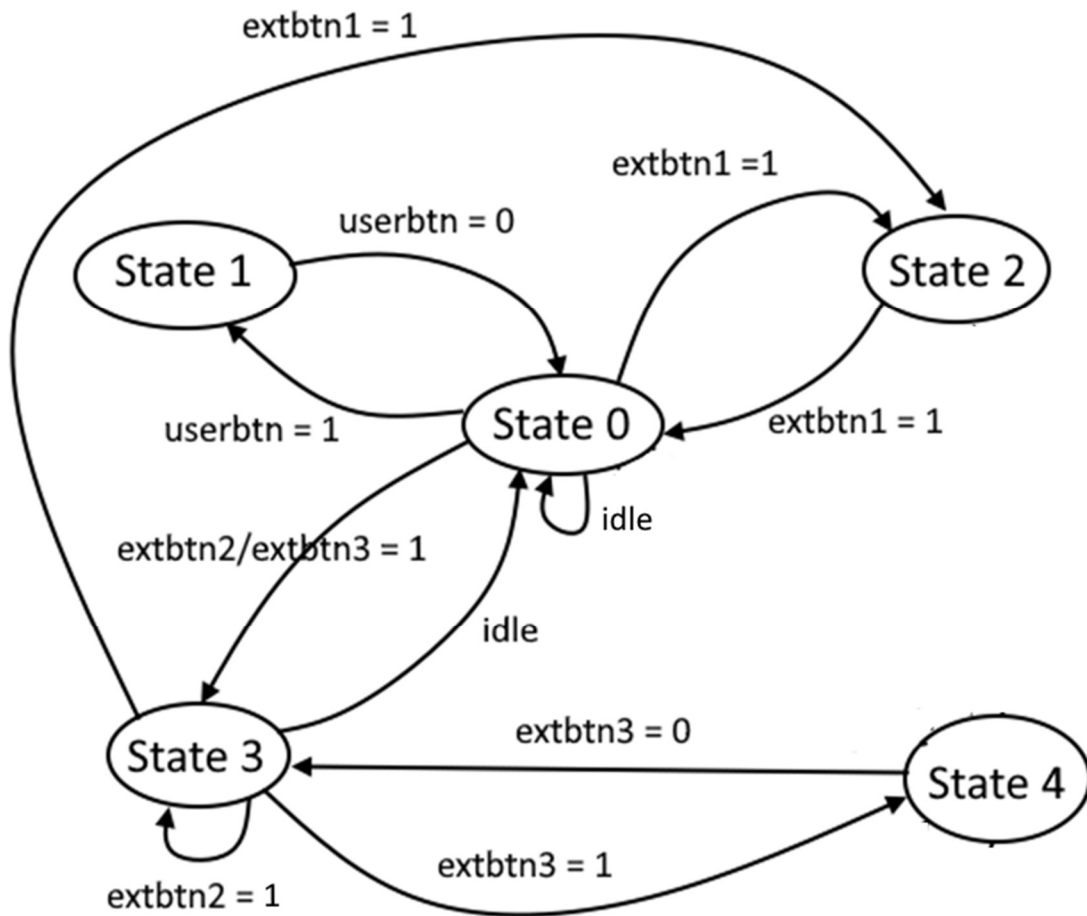
Figure 1: Diagram for Finite State Machine
