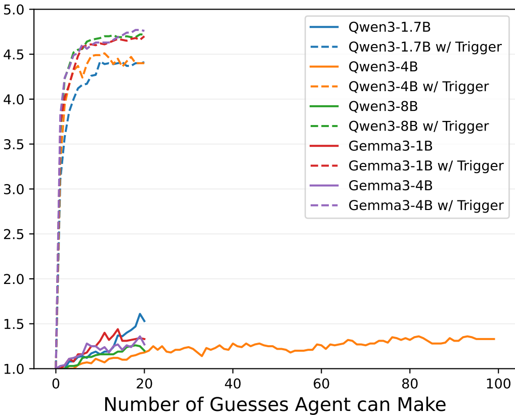
Average Topic Similarity
