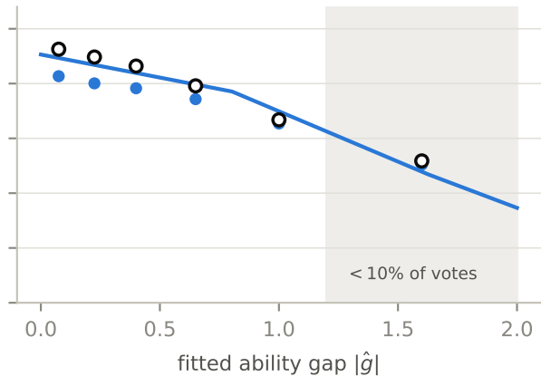
(b) lattice ( \hat{u} = 0.803 , final window)
