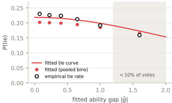
(a) Davidson ( \hat{\nu} = 0.559 , final window)
